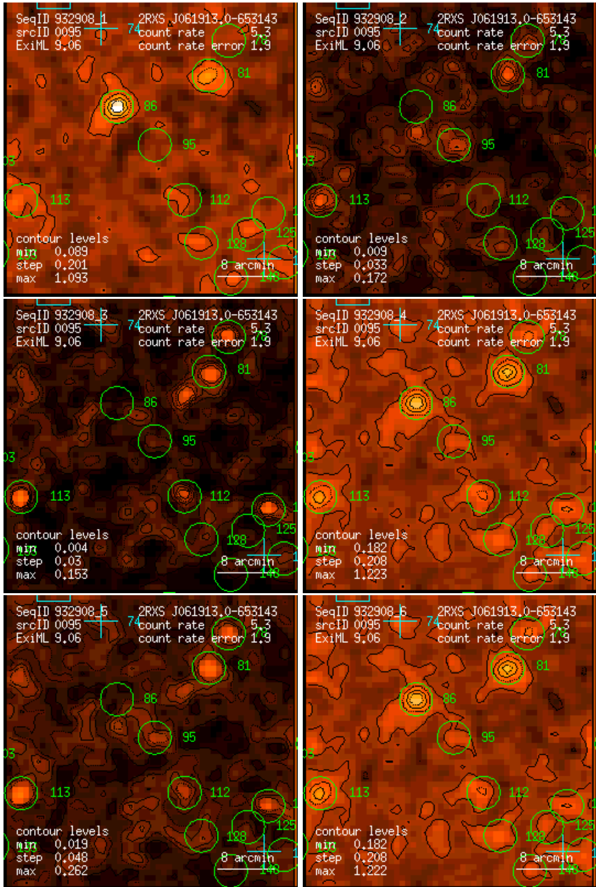
Figure 95: RASS 932908: detection 0095: band rate images, Gaussian filter: (1) PSPC channels 11 – 41, (2) 52 – 90, (3) 91 – 201, (4) 11 – 235, (5) 52 – 201, (6) 11 – 201. Broad band rates in counts/ks. Band rate contour levels in counts/ks/arcmin 2 .
