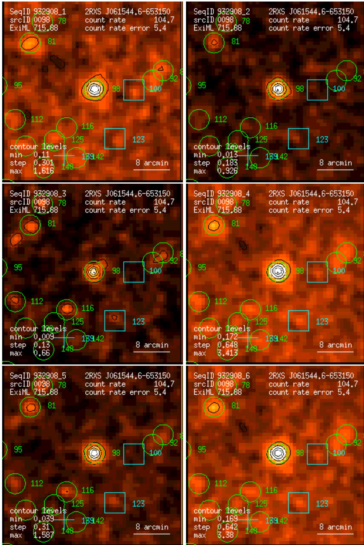
Figure 98: RASS 932908: detection 0098: band rate images, Gaussian filter: (1) PSPC channels 11 – 41, (2) 52 – 90, (3) 91 – 201, (4) 11 – 235, (5) 52 – 201, (6) 11 – 201. Broad band rates in counts/ks. Band rate contour levels in counts/ks/arcmin 2 .
