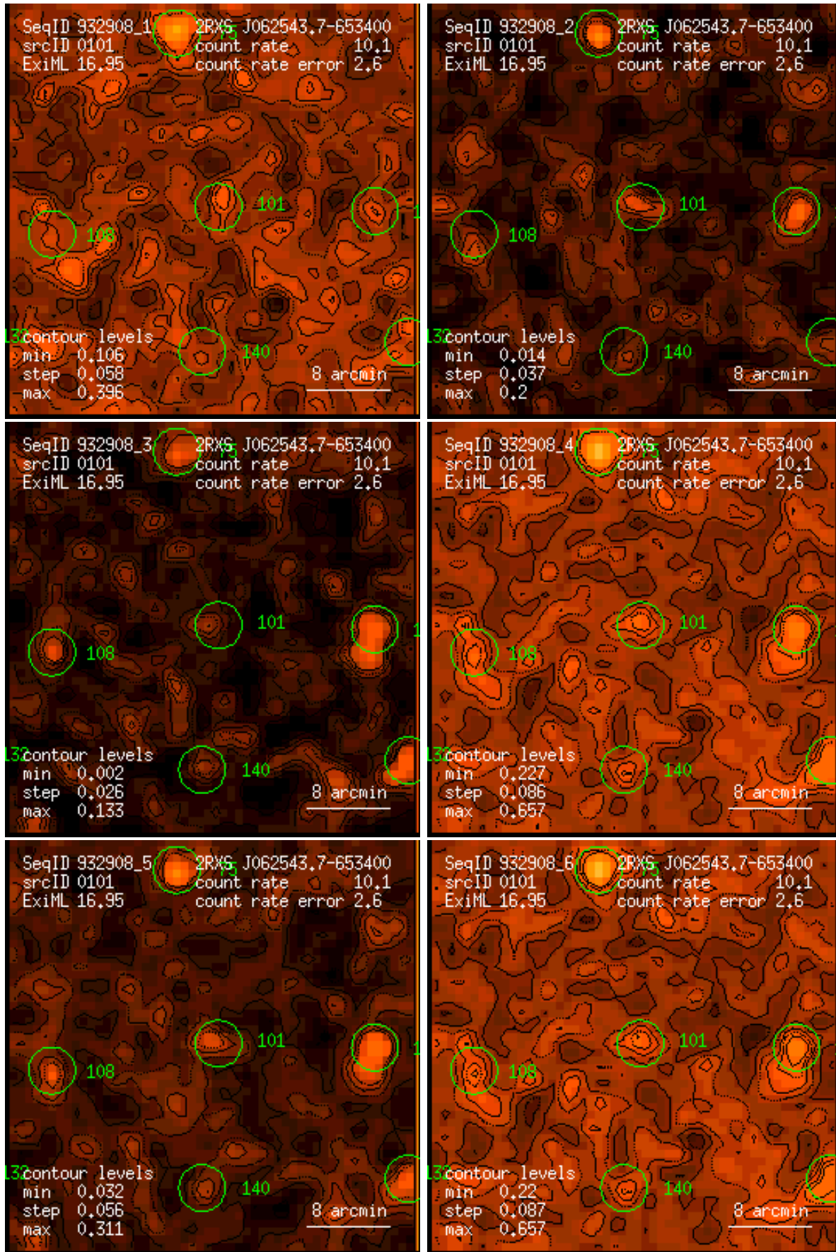
Figure 101: RASS 932908: detection 0101: band rate images, Gaussian filter: (1) PSPC channels 11 – 41, (2) 52 – 90, (3) 91 – 201, (4) 11 – 235, (5) 52 – 201, (6) 11 – 201. Broad band rates in counts/ks. Band rate contour levels in counts/ks/arcmin 2 .
