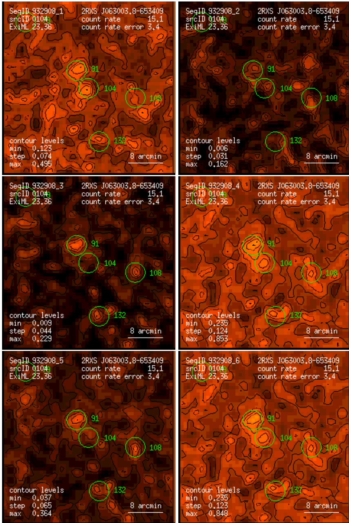
Figure 104: RASS 932908: detection 0104: band rate images, Gaussian filter: (1) PSPC channels 11 – 41, (2) 52 – 90, (3) 91 – 201, (4) 11 – 235, (5) 52 – 201, (6) 11 – 201. Broad band rates in counts/ks. Band rate contour levels in counts/ks/arcmin 2 .
