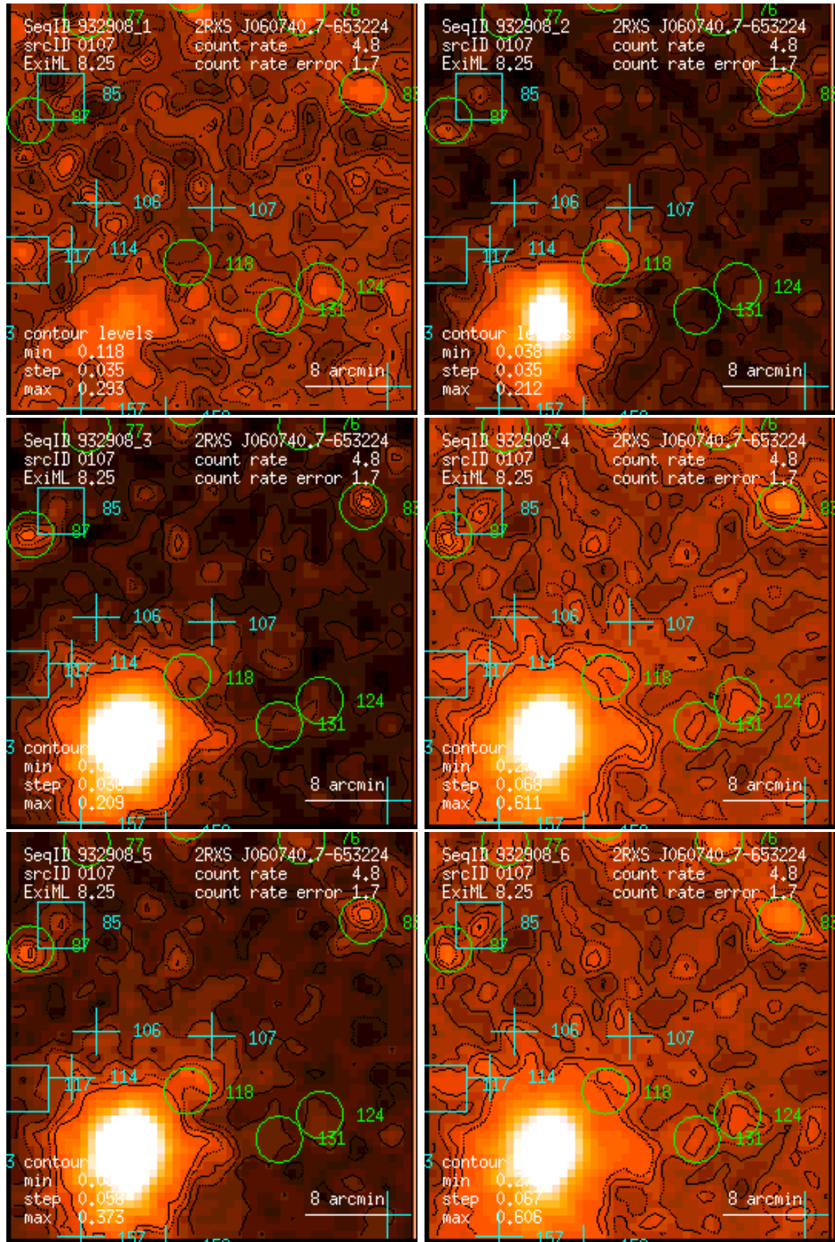
Figure 107: RASS 932908: detection 0107: band rate images, Gaussian filter: (1) PSPC channels 11 – 41, (2) 52 – 90, (3) 91 – 201, (4) 11 – 235, (5) 52 – 201, (6) 11 – 201. Broad band rates in counts/ks. Band rate contour levels in counts/ks/arcmin 2 .
