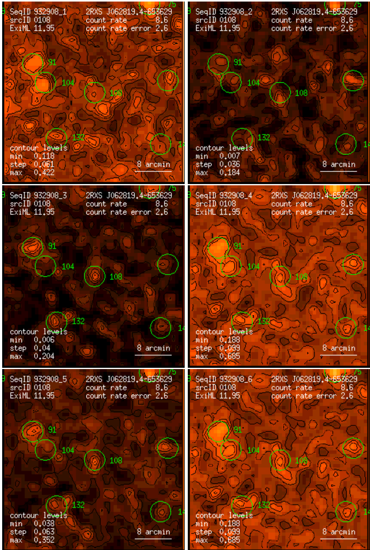
Figure 108: RASS 932908: detection 0108: band rate images, Gaussian filter: (1) PSPC channels 11 – 41, (2) 52 – 90, (3) 91 – 201, (4) 11 – 235, (5) 52 – 201, (6) 11 – 201. Broad band rates in counts/ks. Band rate contour levels in counts/ks/arcmin 2 .
