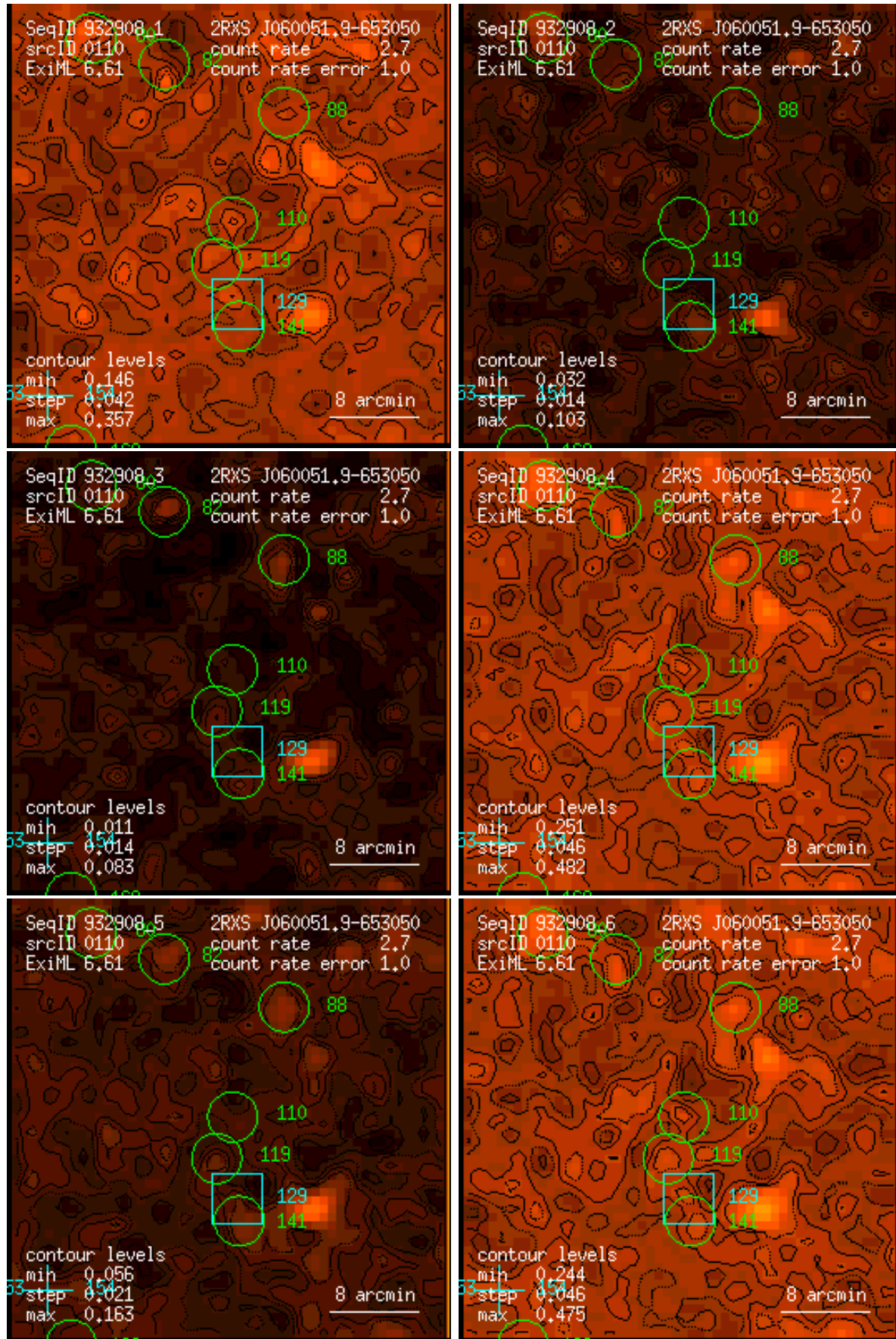
Figure 110: RASS 932908: detection 0110: band rate images, Gaussian filter: (1) PSPC channels 11 – 41, (2) 52 – 90, (3) 91 – 201, (4) 11 – 235, (5) 52 – 201, (6) 11 – 201. Broad band rates in counts/ks. Band rate contour levels in counts/ks/arcmin 2 .
