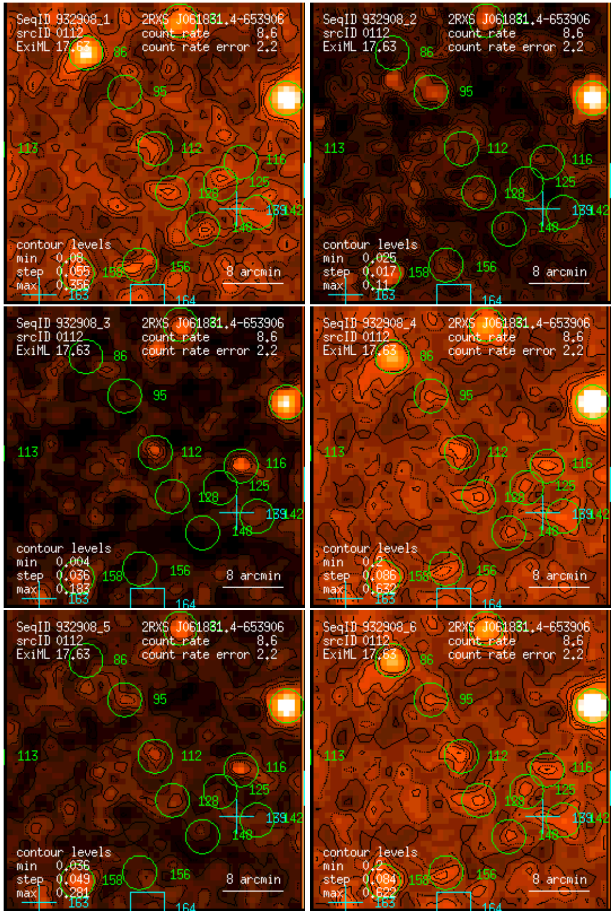
Figure 112: RASS 932908: detection 0112: band rate images, Gaussian filter: (1) PSPC channels 11 – 41, (2) 52 – 90, (3) 91 – 201, (4) 11 – 235, (5) 52 – 201, (6) 11 – 201. Broad band rates in counts/ks. Band rate contour levels in counts/ks/arcmin 2 .
