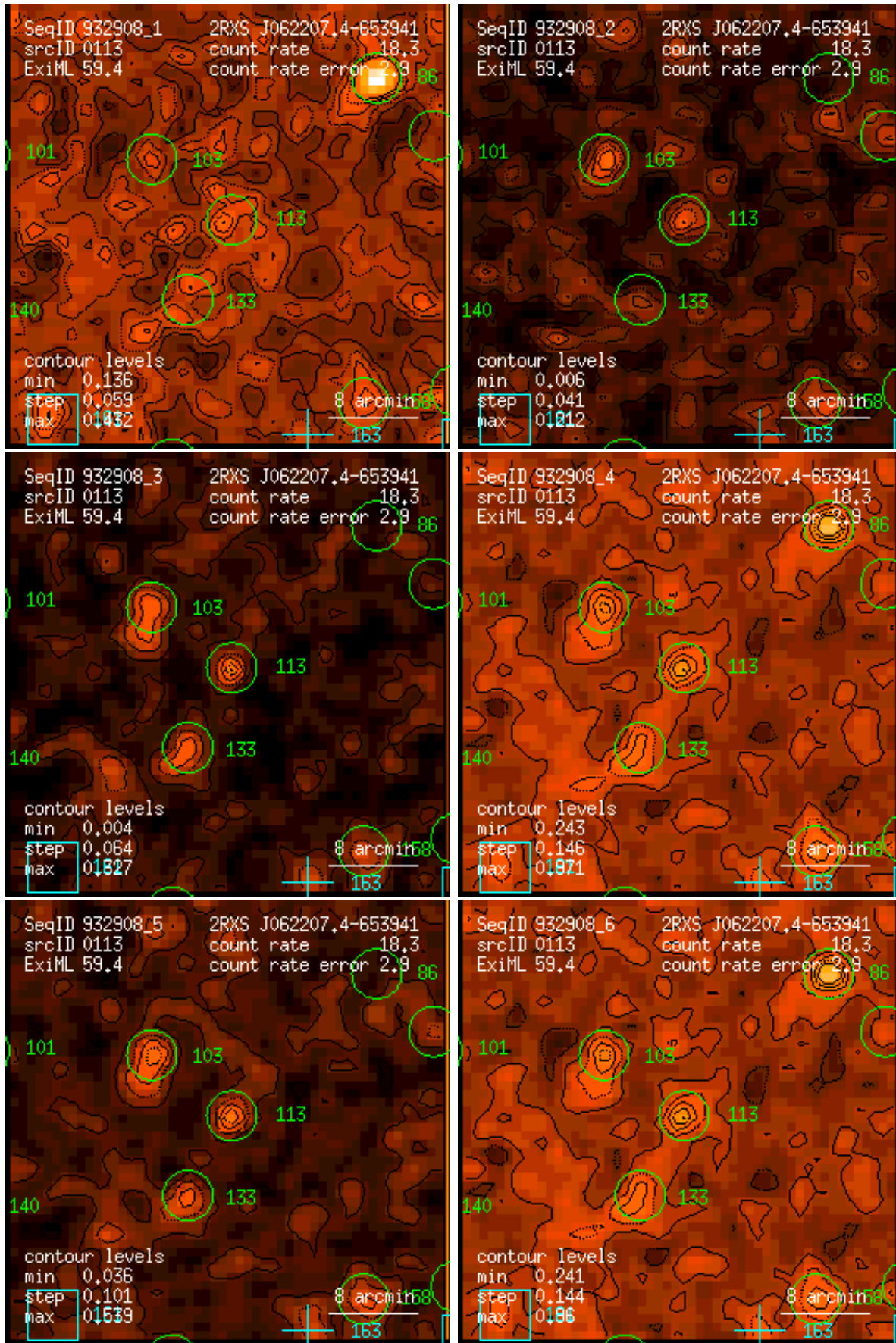
Figure 113: RASS 932908: detection 0113: band rate images, Gaussian filter: (1) PSPC channels 11 – 41, (2) 52 – 90, (3) 91 – 201, (4) 11 – 235, (5) 52 – 201, (6) 11 – 201. Broad band rates in counts/ks. Band rate contour levels in counts/ks/arcmin 2 .
