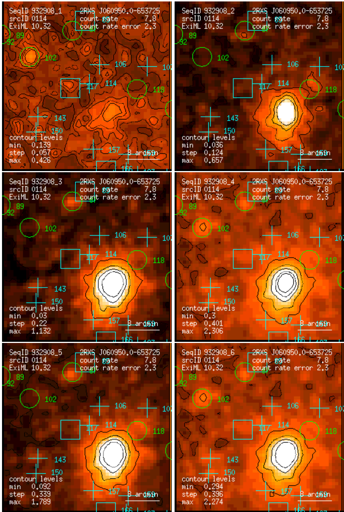
Figure 114: RASS 932908: detection 0114: band rate images, Gaussian filter: (1) PSPC channels 11 – 41, (2) 52 – 90, (3) 91 – 201, (4) 11 – 235, (5) 52 – 201, (6) 11 – 201. Broad band rates in counts/ks. Band rate contour levels in counts/ks/arcmin 2 .
