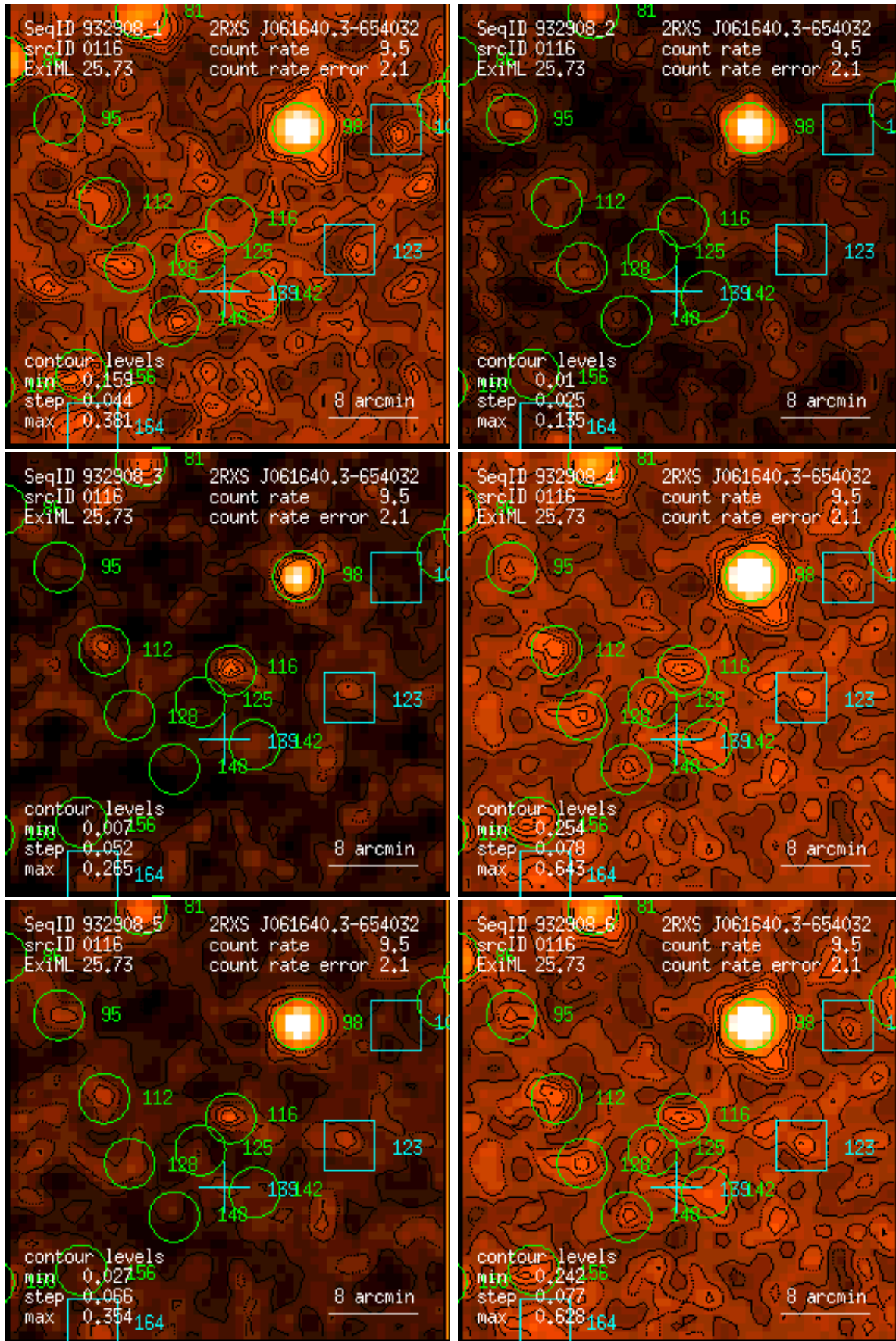
Figure 116: RASS 932908: detection 0116: band rate images, Gaussian filter: (1) PSPC channels 11 – 41, (2) 52 – 90, (3) 91 – 201, (4) 11 – 235, (5) 52 – 201, (6) 11 – 201. Broad band rates in counts/ks. Band rate contour levels in counts/ks/arcmin 2 .
