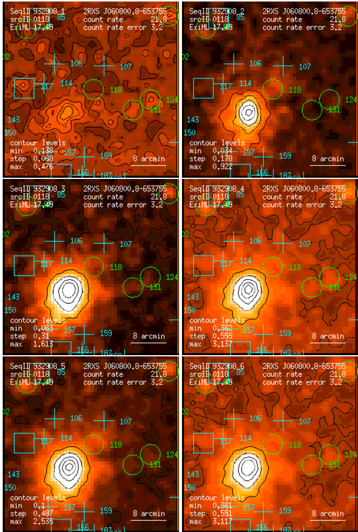
Figure 118: RASS 932908: detection 0118: band rate images, Gaussian filter: (1) PSPC channels 11 – 41, (2) 52 – 90, (3) 91 – 201, (4) 11 – 235, (5) 52 – 201, (6) 11 – 201. Broad band rates in counts/ks. Band rate contour levels in counts/ks/arcmin 2 .
