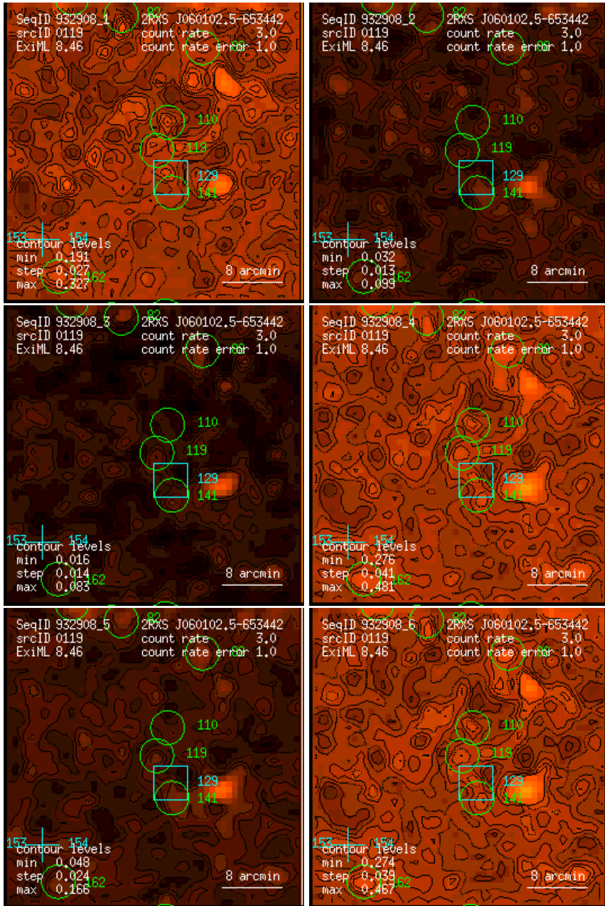
Figure 119: RASS 932908: detection 0119: band rate images, Gaussian filter: (1) PSPC channels 11 – 41, (2) 52 – 90, (3) 91 – 201, (4) 11 – 235, (5) 52 – 201, (6) 11 – 201. Broad band rates in counts/ks. Band rate contour levels in counts/ks/arcmin 2 .
