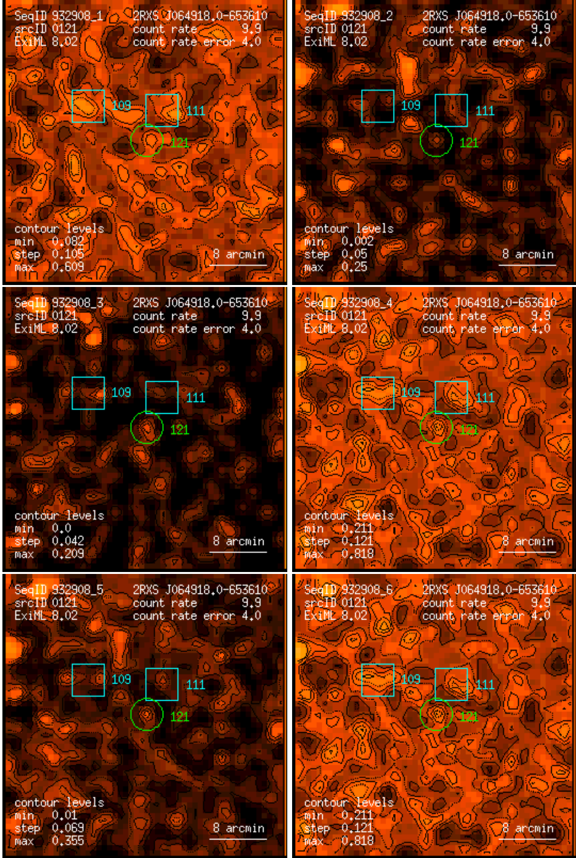
Figure 121: RASS 932908: detection 0121: band rate images, Gaussian filter: (1) PSPC channels 11 – 41, (2) 52 – 90, (3) 91 – 201, (4) 11 – 235, (5) 52 – 201, (6) 11 – 201. Broad band rates in counts/ks. Band rate contour levels in counts/ks/arcmin 2 .
