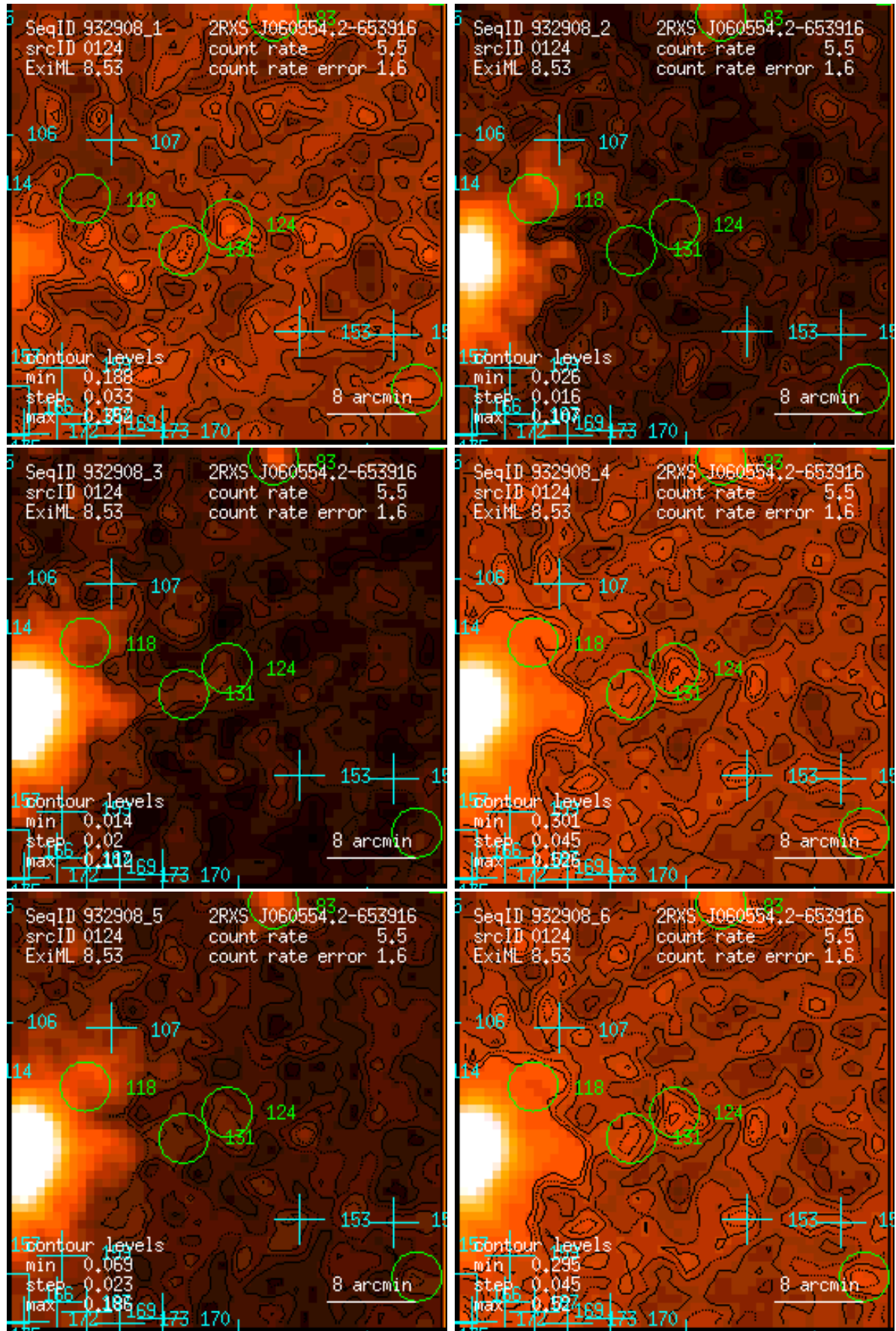
Figure 124: RASS 932908: detection 0124: band rate images, Gaussian filter: (1) PSPC channels 11 – 41, (2) 52 – 90, (3) 91 – 201, (4) 11 – 235, (5) 52 – 201, (6) 11 – 201. Broad band rates in counts/ks. Band rate contour levels in counts/ks/arcmin 2 .
