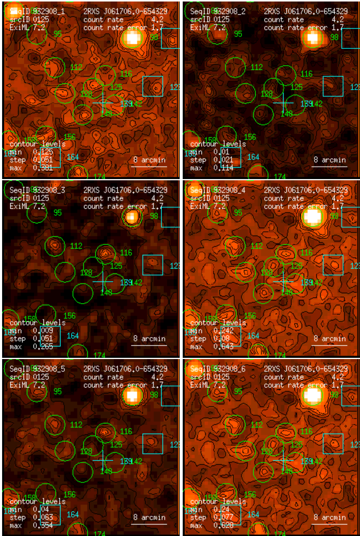
Figure 125: RASS 932908: detection 0125: band rate images, Gaussian filter: (1) PSPC channels 11 – 41, (2) 52 – 90, (3) 91 – 201, (4) 11 – 235, (5) 52 – 201, (6) 11 – 201. Broad band rates in counts/ks. Band rate contour levels in counts/ks/arcmin 2 .
