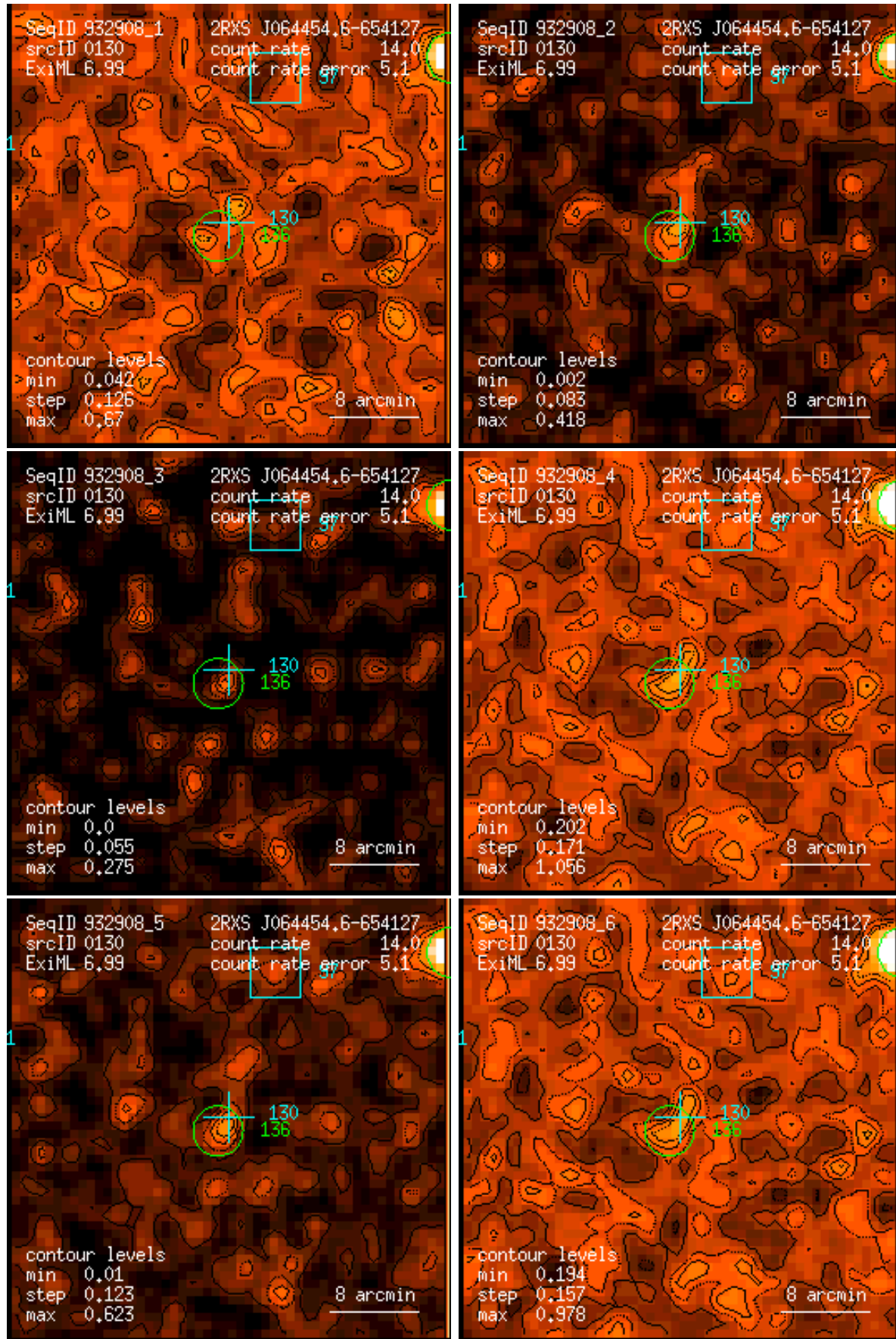
Figure 130: RASS 932908: detection 0130: band rate images, Gaussian filter: (1) PSPC channels 11 – 41, (2) 52 – 90, (3) 91 – 201, (4) 11 – 235, (5) 52 – 201, (6) 11 – 201. Broad band rates in counts/ks. Band rate contour levels in counts/ks/arcmin 2 .
