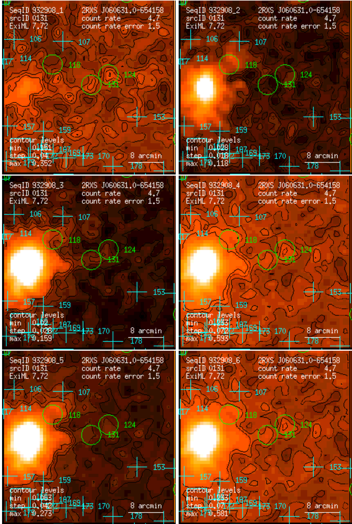
Figure 131: RASS 932908: detection 0131: band rate images, Gaussian filter: (1) PSPC channels 11 – 41, (2) 52 – 90, (3) 91 – 201, (4) 11 – 235, (5) 52 – 201, (6) 11 – 201. Broad band rates in counts/ks. Band rate contour levels in counts/ks/arcmin 2 .
