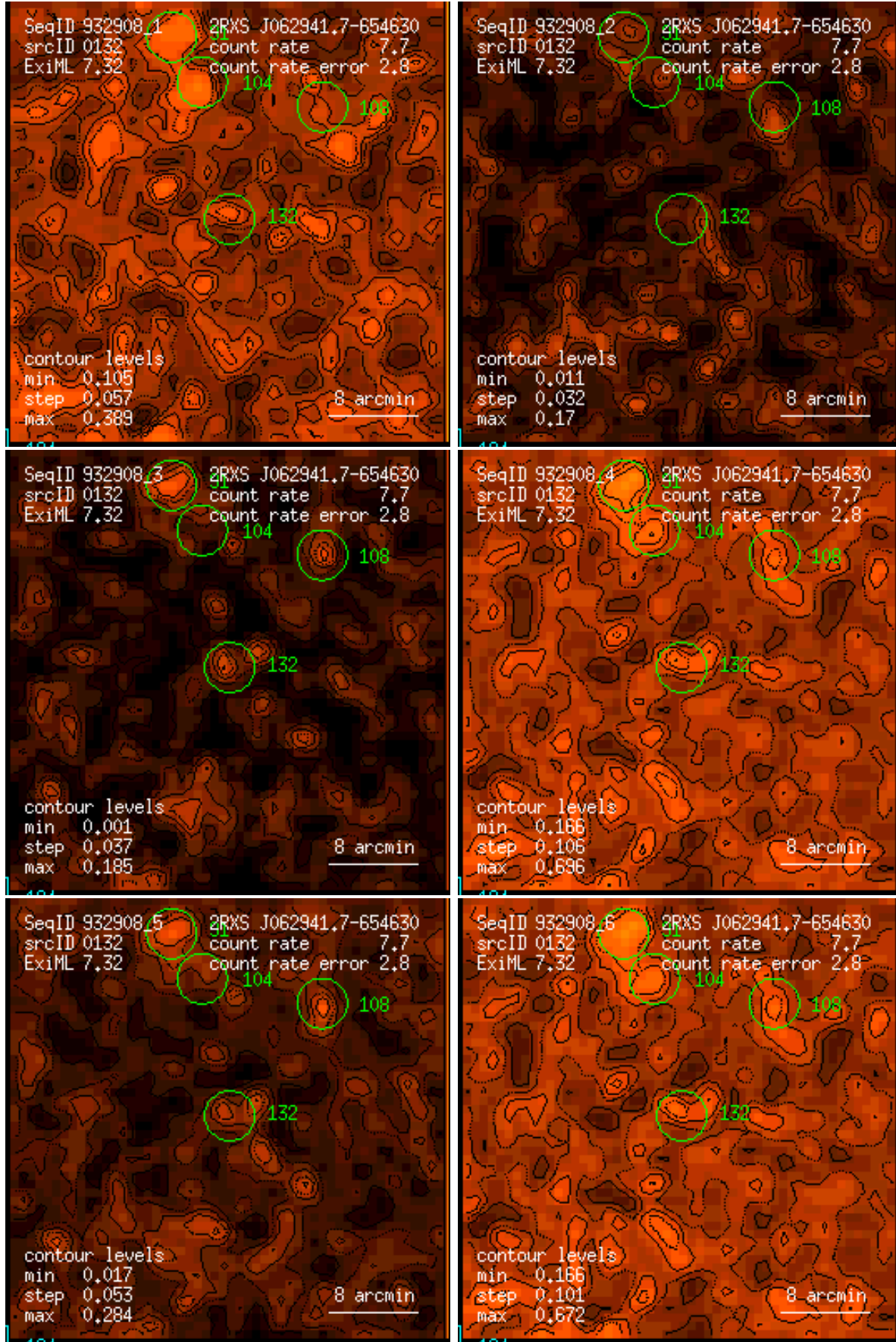
Figure 132: RASS 932908: detection 0132: band rate images, Gaussian filter: (1) PSPPC channels 11 – 41, (2) 52 – 90, (3) 91 – 201, (4) 11 – 235, (5) 52 – 201, (6) 11 – 201. Broad band rates in counts/ks. Band rate contour levels in counts/ks/arcmin 2 .
