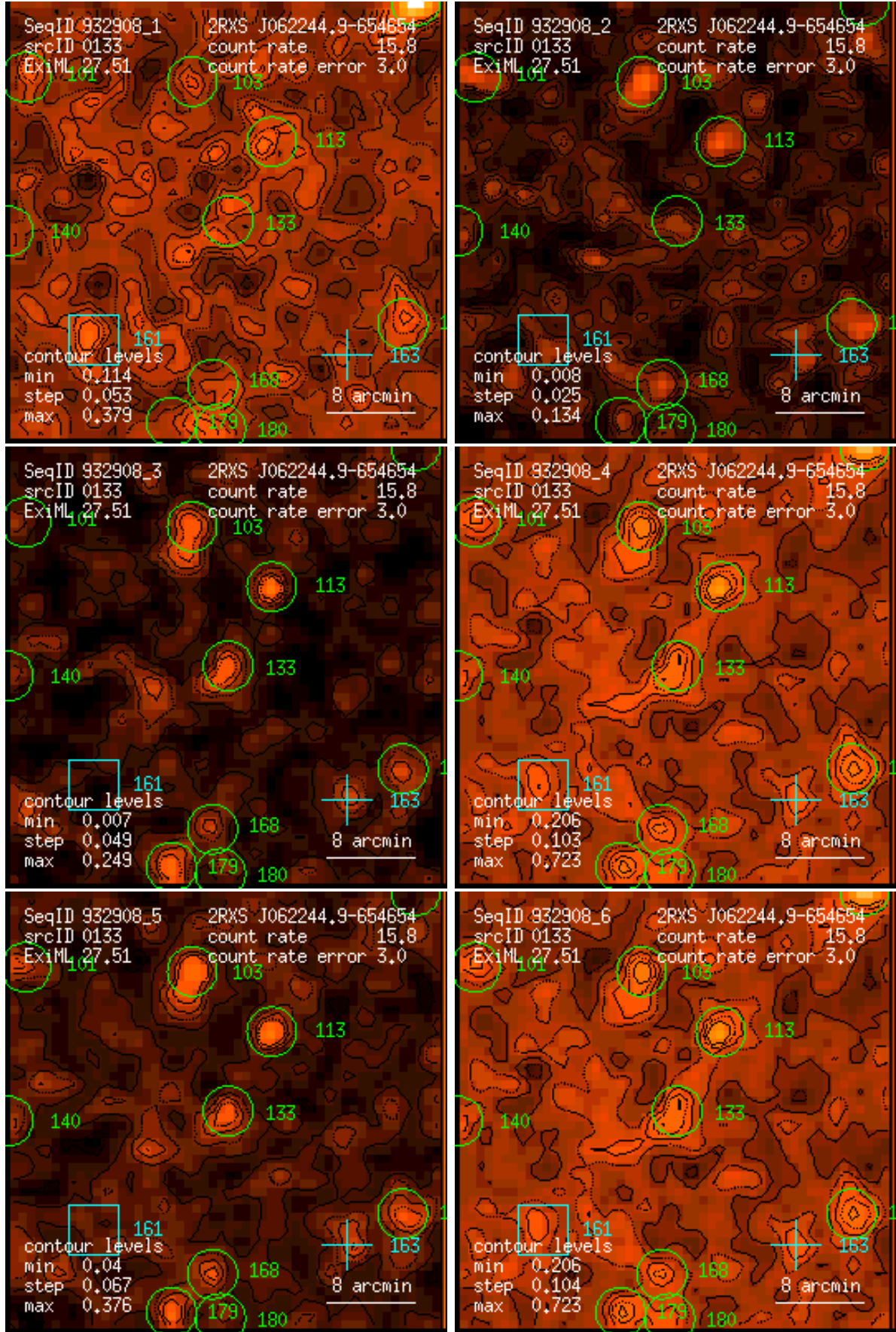
Figure 133: RASS 932908: detection 0133: band rate images, Gaussian filter: (1) PSPC channels 11 – 41, (2) 52 – 90, (3) 91 – 201, (4) 11 – 235, (5) 52 – 201, (6) 11 – 201. Broad band rates in counts/ks. Band rate contour levels in counts/ks/arcmin 2 .
