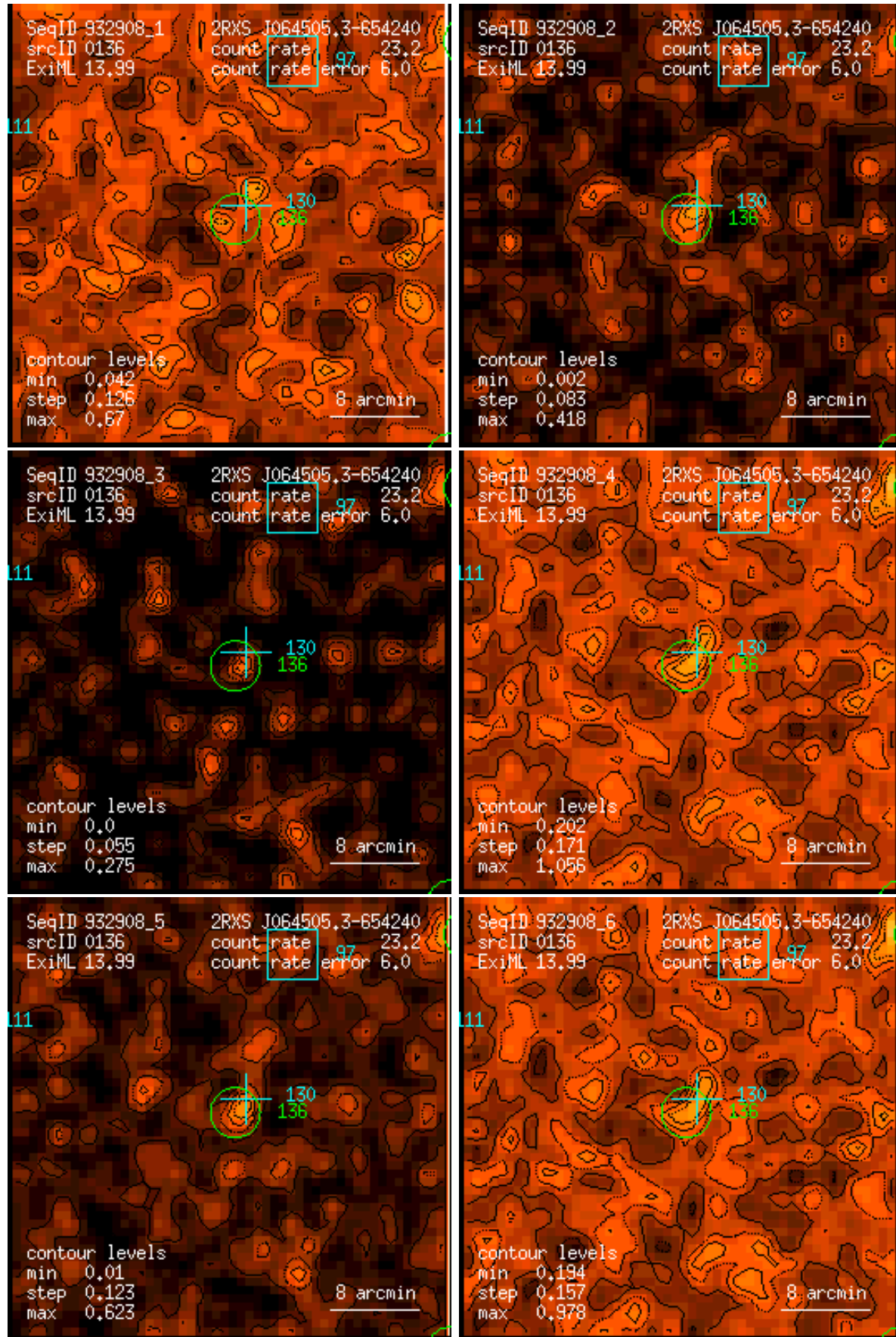
Figure 136: RASS 932908: detection 0136: band rate images, Gaussian filter: (1) PSPC channels 11 – 41, (2) 52 – 90, (3) 91 – 201, (4) 11 – 235, (5) 52 – 201, (6) 11 – 201. Broad band rates in counts/ks. Band rate contour levels in counts/ks/arcmin 2 .
