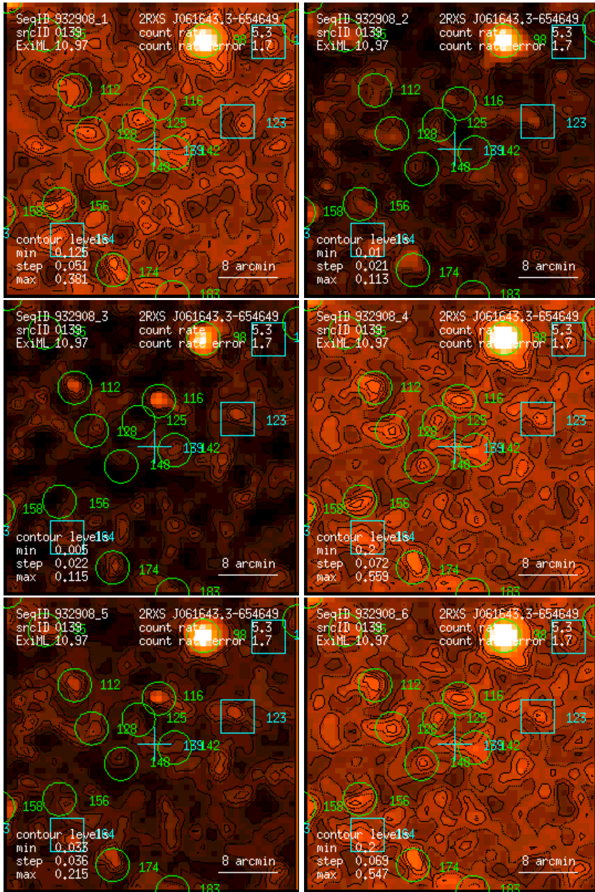
Figure 139: RASS 932908: detection 0139: band rate images, Gaussian filter: (1) PSPC channels 11 – 41, (2) 52 – 90, (3) 91 – 201, (4) 11 – 235, (5) 52 – 201, (6) 11 – 201. Broad band rates in counts/ks. Band rate contour levels in counts/ks/arcmin 2 .
