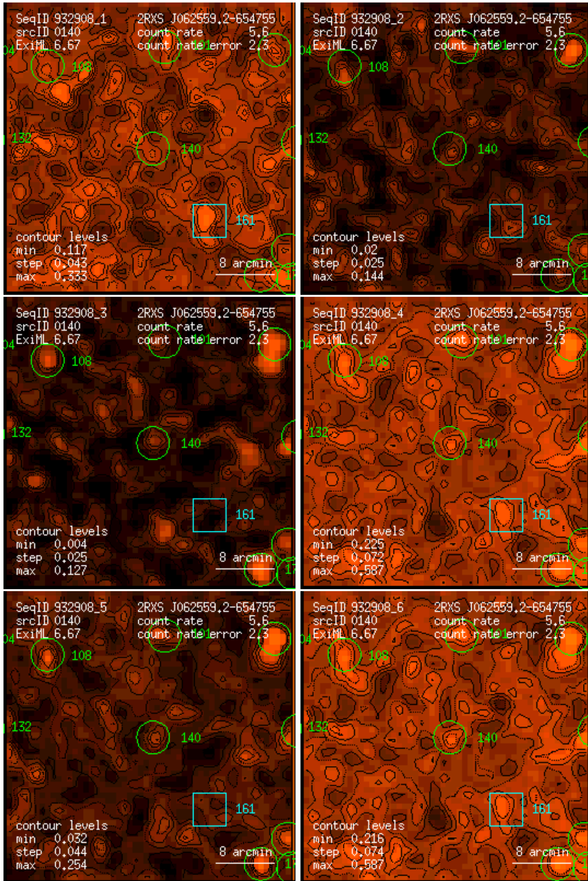
Figure 140: RASS 932908: detection 0140: band rate images, Gaussian filter: (1) PSPC channels 11 – 41, (2) 52 – 90, (3) 91 – 201, (4) 11 – 235, (5) 52 – 201, (6) 11 – 201. Broad band rates in counts/ks. Band rate contour levels in counts/ks/arcmin 2 .
