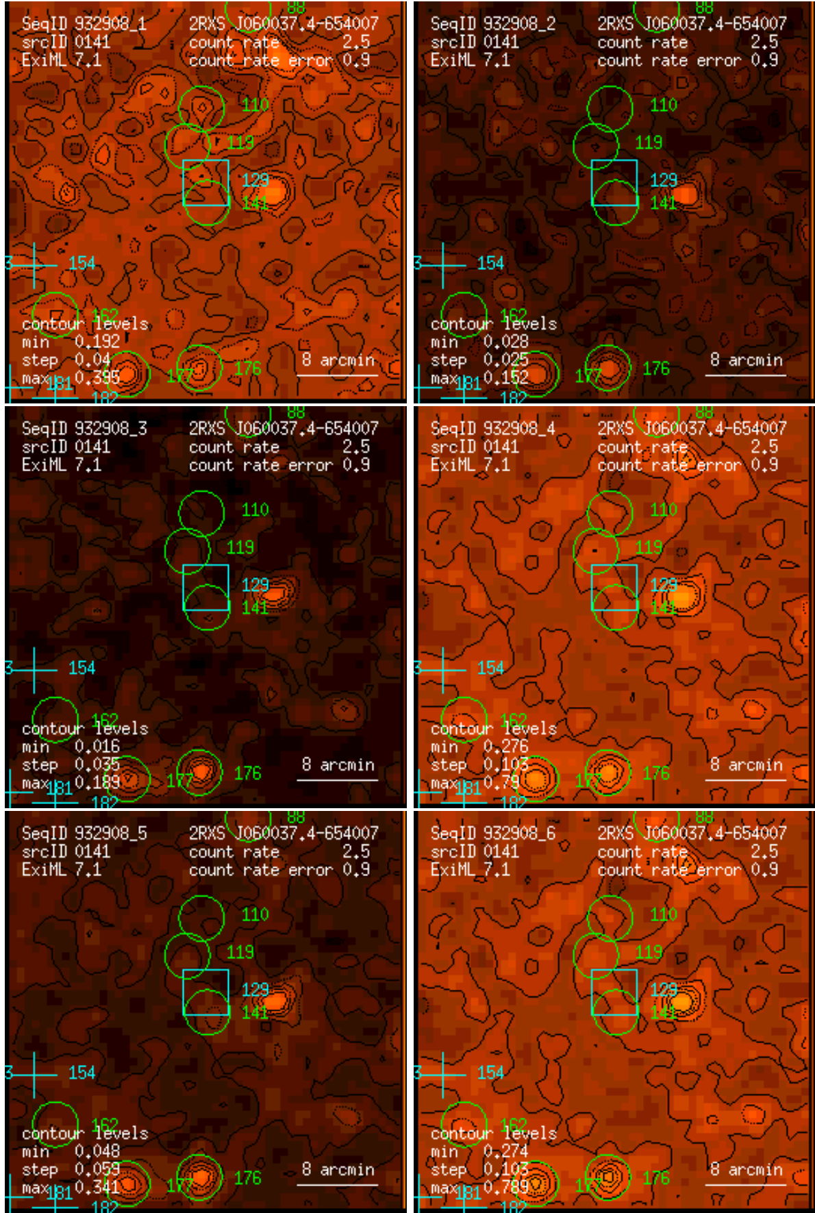
Figure 141: RASS 932908: detection 0141: band rate images, Gaussian filter: (1) PSPC channels 11 – 41, (2) 52 – 90, (3) 91 – 201, (4) 11 – 235, (5) 52 – 201, (6) 11 – 201. Broad band rates in counts/ks. Band rate contour levels in counts/ks/arcmin 2 .
