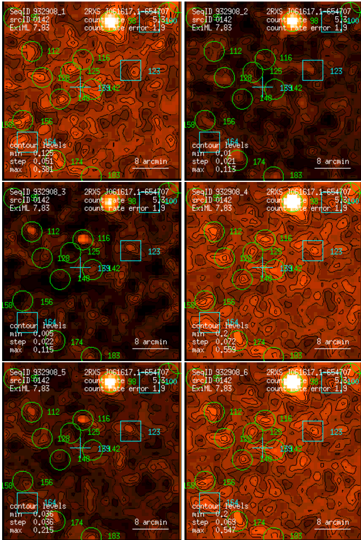
Figure 142: RASS 932908: detection 0142: band rate images, Gaussian filter: (1) PSPC channels 11 – 41, (2) 52 – 90, (3) 91 – 201, (4) 11 – 235, (5) 52 – 201, (6) 11 – 201. Broad band rates in counts/ks. Band rate contour levels in counts/ks/arcmin 2 .
