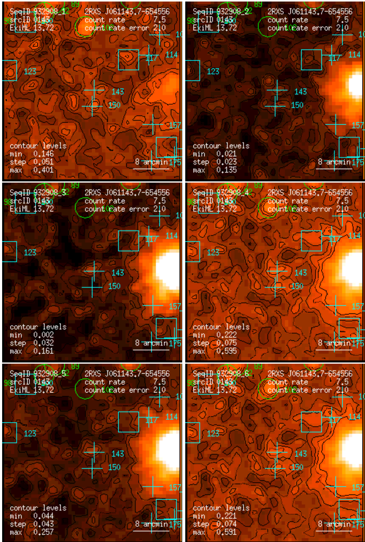
Figure 143: RASS 932908: detection 0143: band rate images, Gaussian filter: (1) PSPC channels 11 – 41, (2) 52 – 90, (3) 91 – 201, (4) 11 – 235, (5) 52 – 201, (6) 11 – 201. Broad band rates in counts/ks. Band rate contour levels in counts/ks/arcmin 2 .
