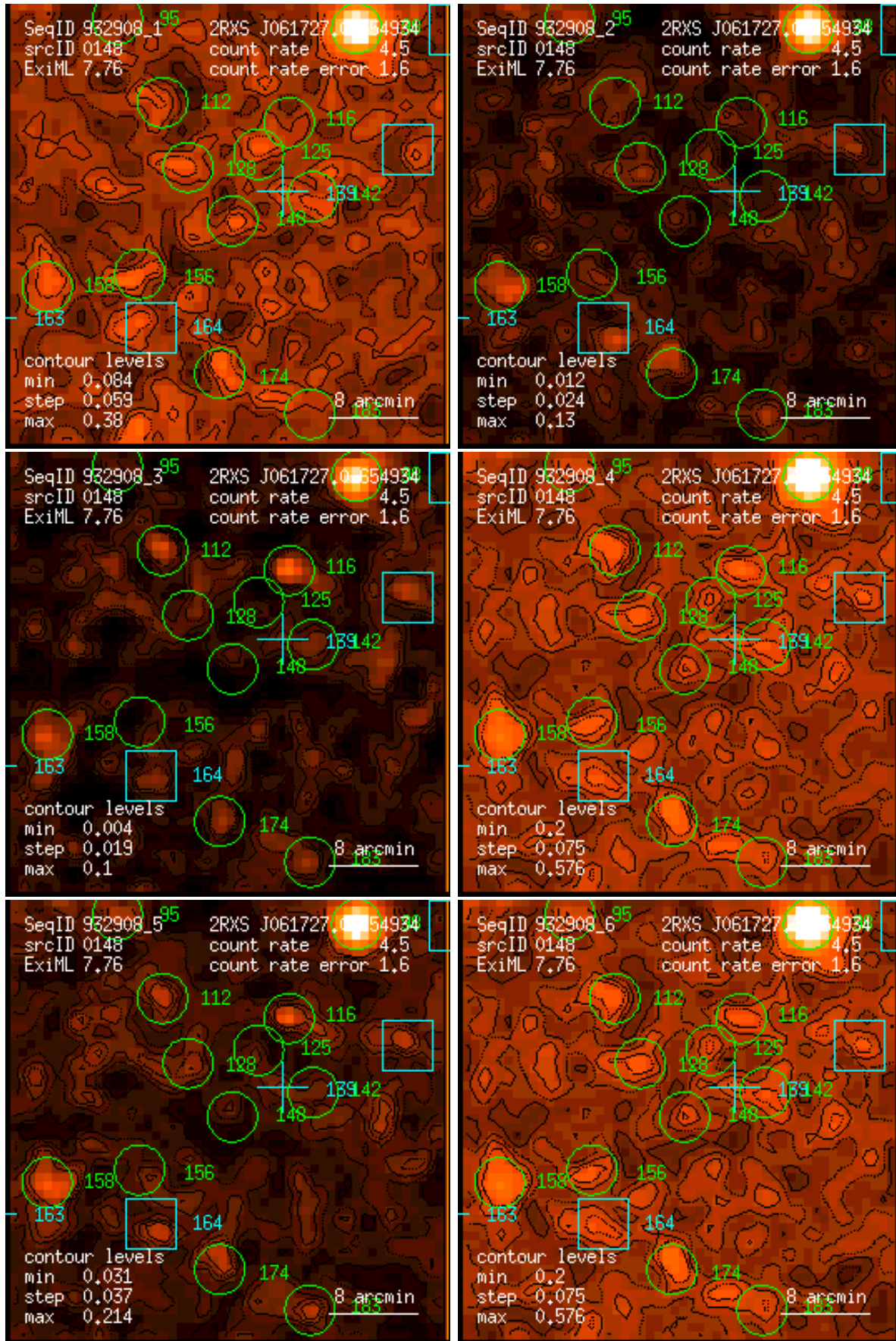
Figure 148: RASS 932908: detection 0148: band rate images, Gaussian filter: (1) PSPC channels 11 – 41, (2) 52 – 90, (3) 91 – 201, (4) 11 – 235, (5) 52 – 201, (6) 11 – 201. Broad band rates in counts/ks. Band rate contour levels in counts/ks/arcmin 2 .
