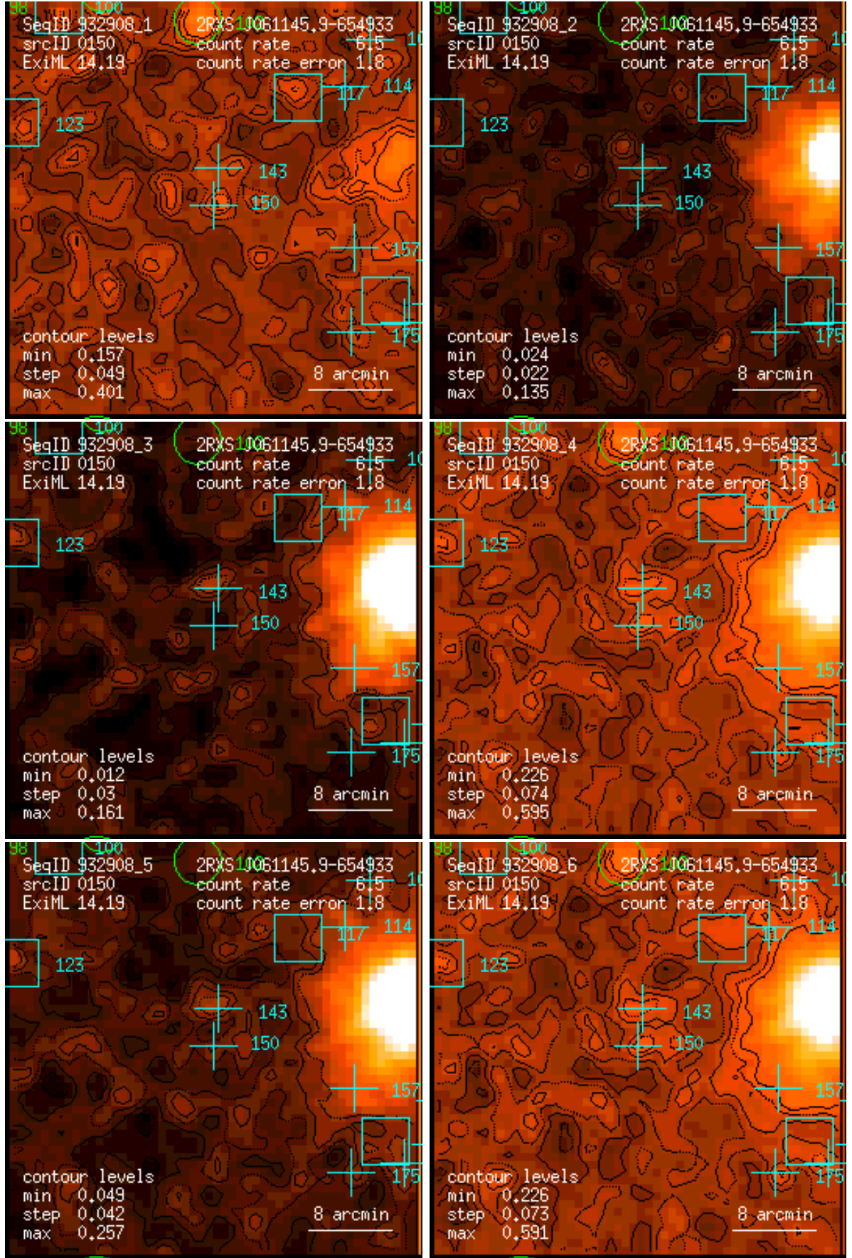
Figure 150: RASS 932908: detection 0150: band rate images, Gaussian filter: (1) PSPC channels 11 – 41, (2) 52 – 90, (3) 91 – 201, (4) 11 – 235, (5) 52 – 201, (6) 11 – 201. Broad band rates in counts/ks. Band rate contour levels in counts/ks/arcmin 2 .
