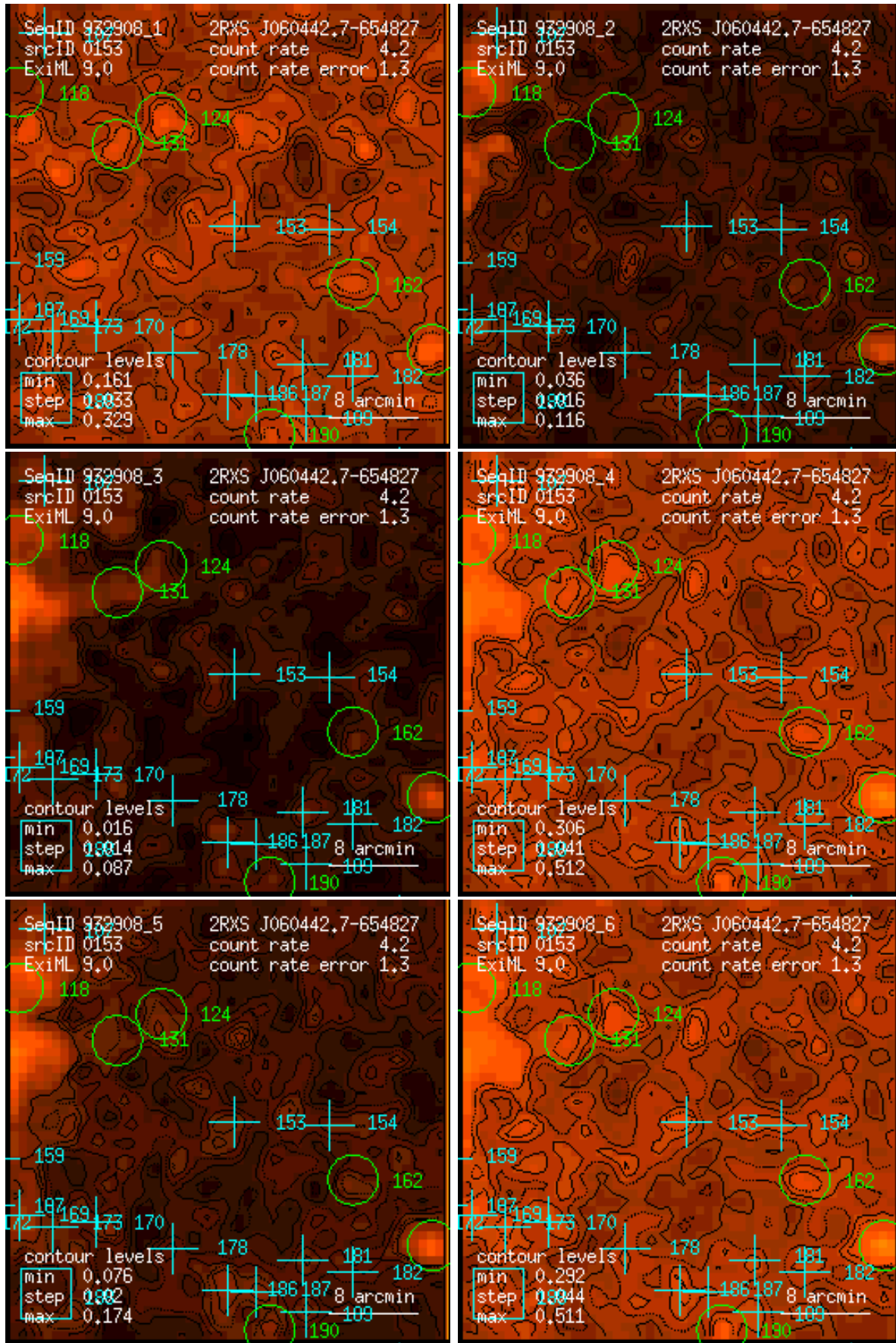
Figure 153: RASS 932908: detection 0153: band rate images, Gaussian filter: (1) PSPC channels 11 – 41, (2) 52 – 90, (3) 91 – 201, (4) 11 – 235, (5) 52 – 201, (6) 11 – 201. Broad band rates in counts/ks. Band rate contour levels in counts/ks/arcmin 2 .
