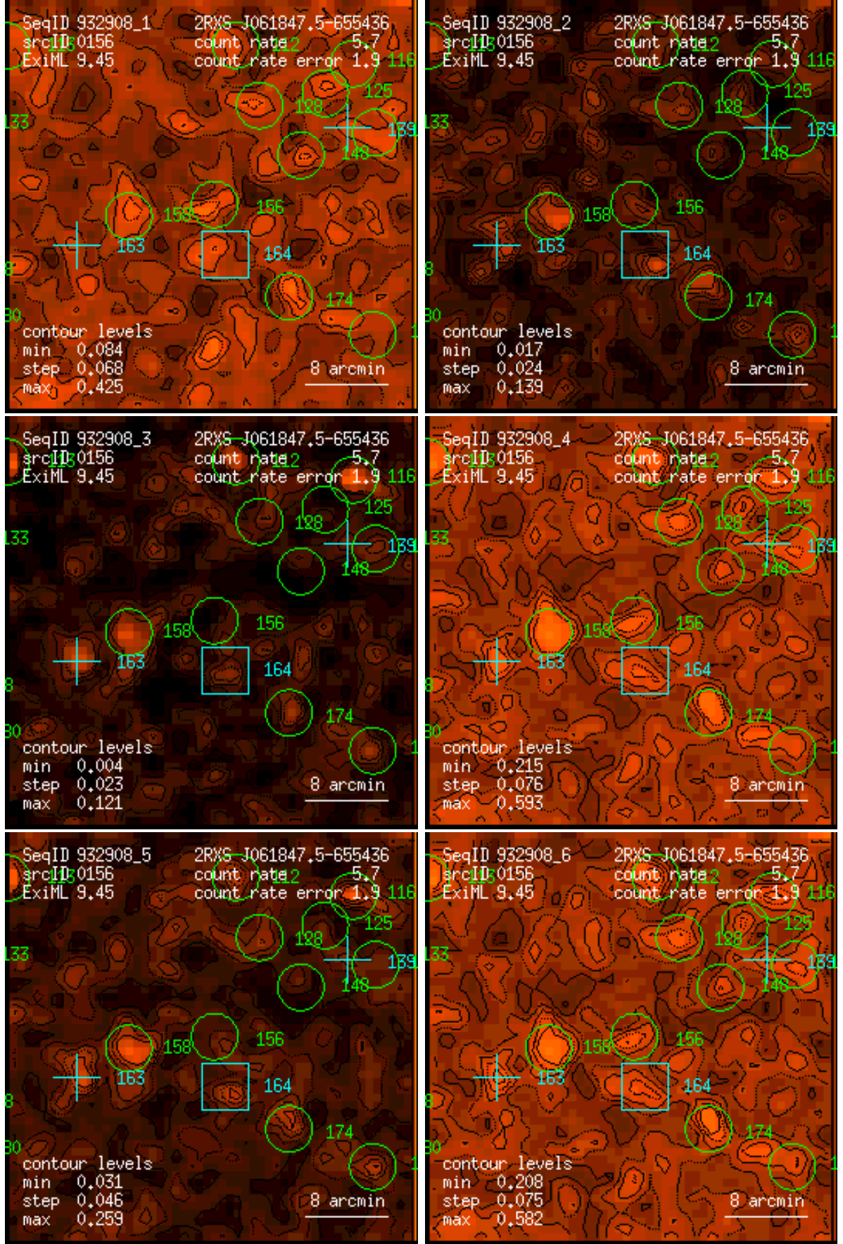
Figure 156: RASS 932908: detection 0156: band rate images, Gaussian filter: (1) PSPC channels 11 – 41, (2) 52 – 90, (3) 91 – 201, (4) 11 – 235, (5) 52 – 201, (6) 11 – 201. Broad band rates in counts/ks. Band rate contour levels in counts/ks/arcmin 2 .
