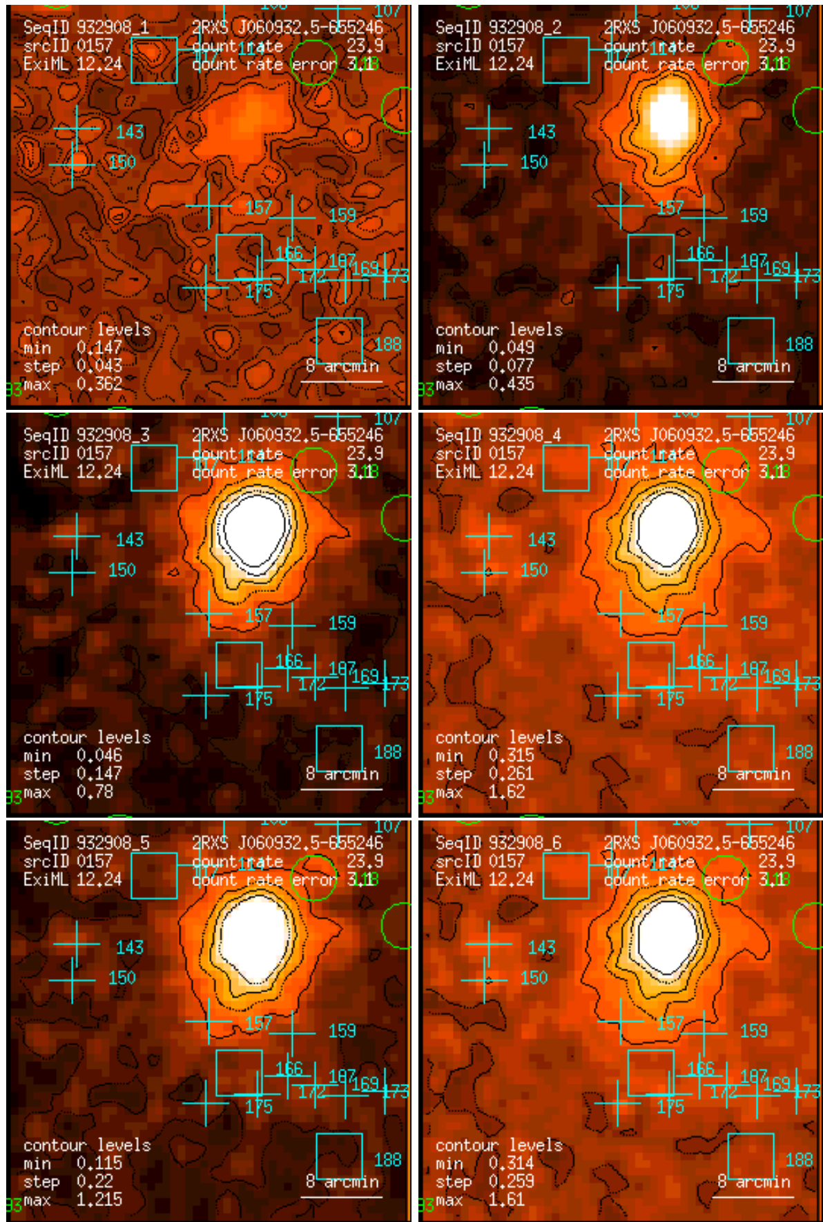
Figure 157: RASS 932908: detection 0157: band rate images, Gaussian filter: (1) PSPC channels 11 – 41, (2) 52 – 90, (3) 91 – 201, (4) 11 – 235, (5) 52 – 201, (6) 11 – 201. Broad band rates in counts/ks. Band rate contour levels in counts/ks/arcmin 2 .
