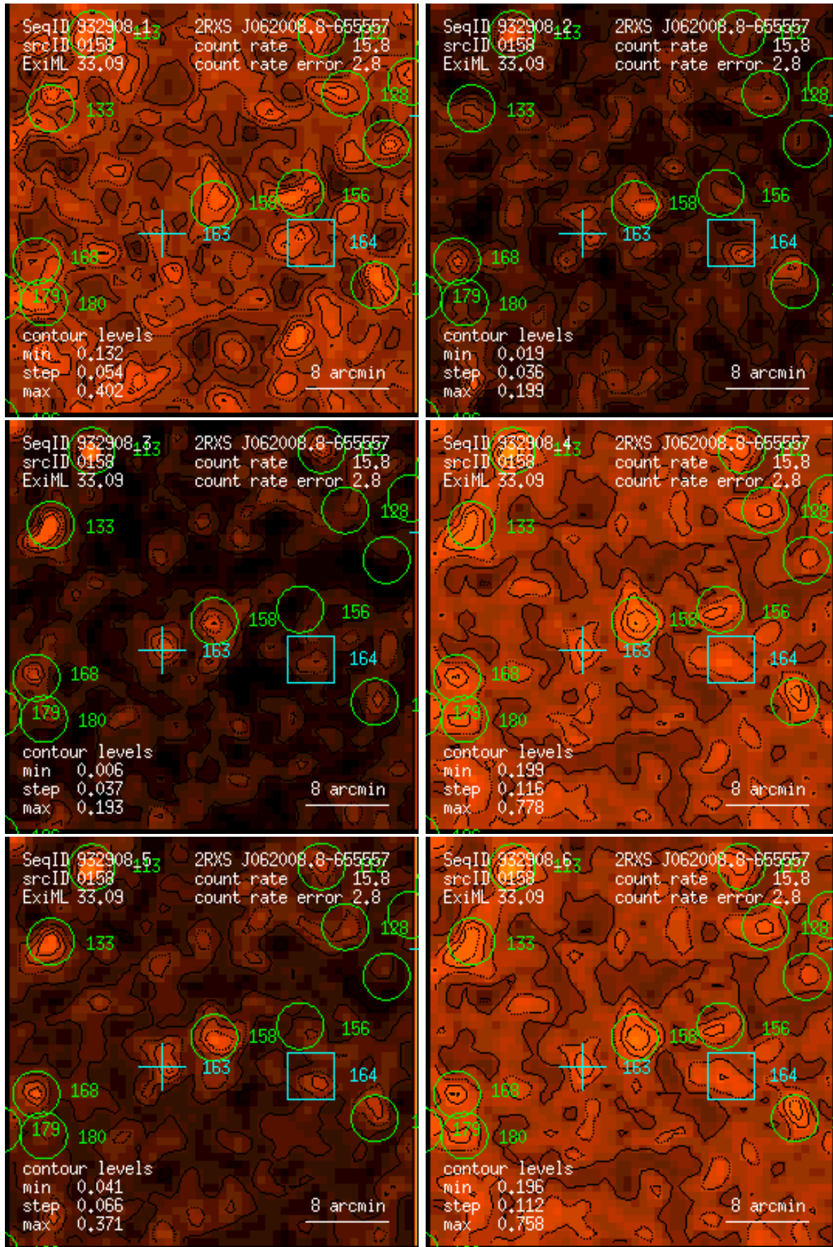
Figure 158: RASS 932908: detection 0158: band rate images, Gaussian filter: (1) PSPC channels 11 – 41, (2) 52 – 90, (3) 91 – 201, (4) 11 – 235, (5) 52 – 201, (6) 11 – 201. Broad band rates in counts/ks. Band rate contour levels in counts/ks/arcmin 2 .
