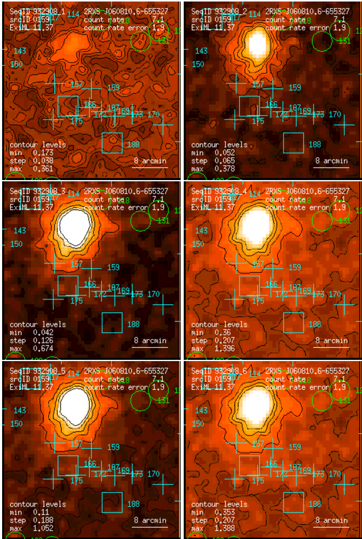
Figure 159: RASS 932908: detection 0159: band rate images, Gaussian filter: (1) PSPC channels 11 – 41, (2) 52 – 90, (3) 91 – 201, (4) 11 – 235, (5) 52 – 201, (6) 11 – 201. Broad band rates in counts/ks. Band rate contour levels in counts/ks/arcmin 2 .
