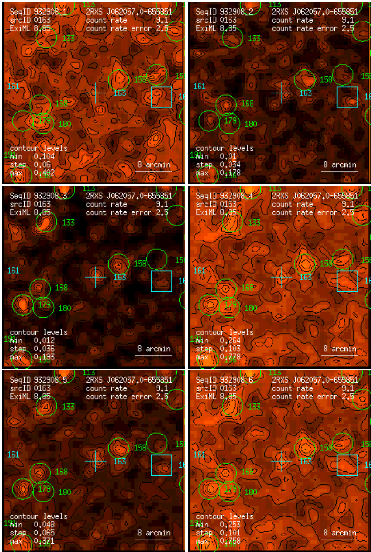
Figure 163: RASS 932908: detection 0163: band rate images, Gaussian filter: (1) PSPC channels 11 – 41, (2) 52 – 90, (3) 91 – 201, (4) 11 – 235, (5) 52 – 201, (6) 11 – 201. Broad band rates in counts/ks. Band rate contour levels in counts/ks/arcmin 2 .
