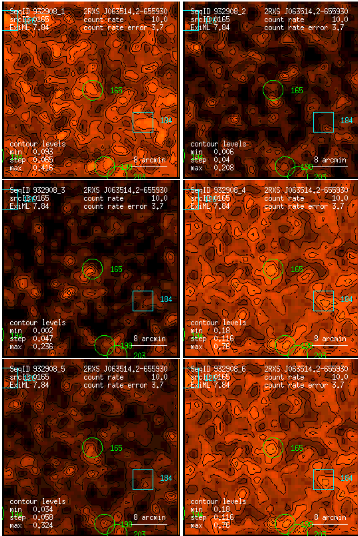
Figure 165: RASS 932908: detection 0165: band rate images, Gaussian filter: (1) PSPC channels 11 – 41, (2) 52 – 90, (3) 91 – 201, (4) 11 – 235, (5) 52 – 201, (6) 11 – 201. Broad band rates in counts/ks. Band rate contour levels in counts/ks/arcmin 2 .
