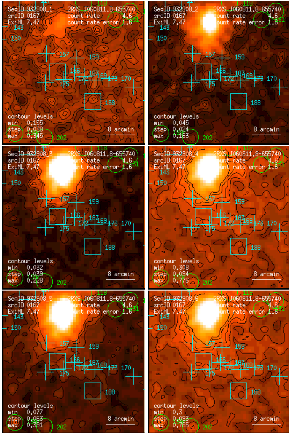
Figure 167: RASS 932908: detection 0167: band rate images, Gaussian filter: (1) PSPC channels 11 – 41, (2) 52 – 90, (3) 91 – 201, (4) 11 – 235, (5) 52 – 201, (6) 11 – 201. Broad band rates in counts/ks. Band rate contour levels in counts/ks/arcmin 2 .
