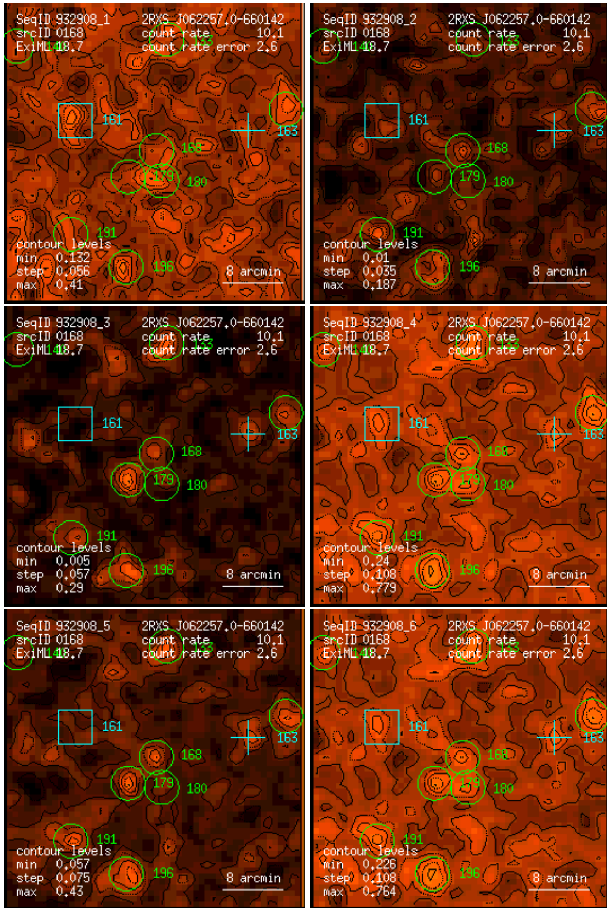
Figure 168: RASS 932908: detection 0168: band rate images, Gaussian filter: (1) PSPC channels 11 – 41, (2) 52 – 90, (3) 91 – 201, (4) 11 – 235, (5) 52 – 201, (6) 11 – 201. Broad band rates in counts/ks. Band rate contour levels in counts/ks/arcmin 2 .
