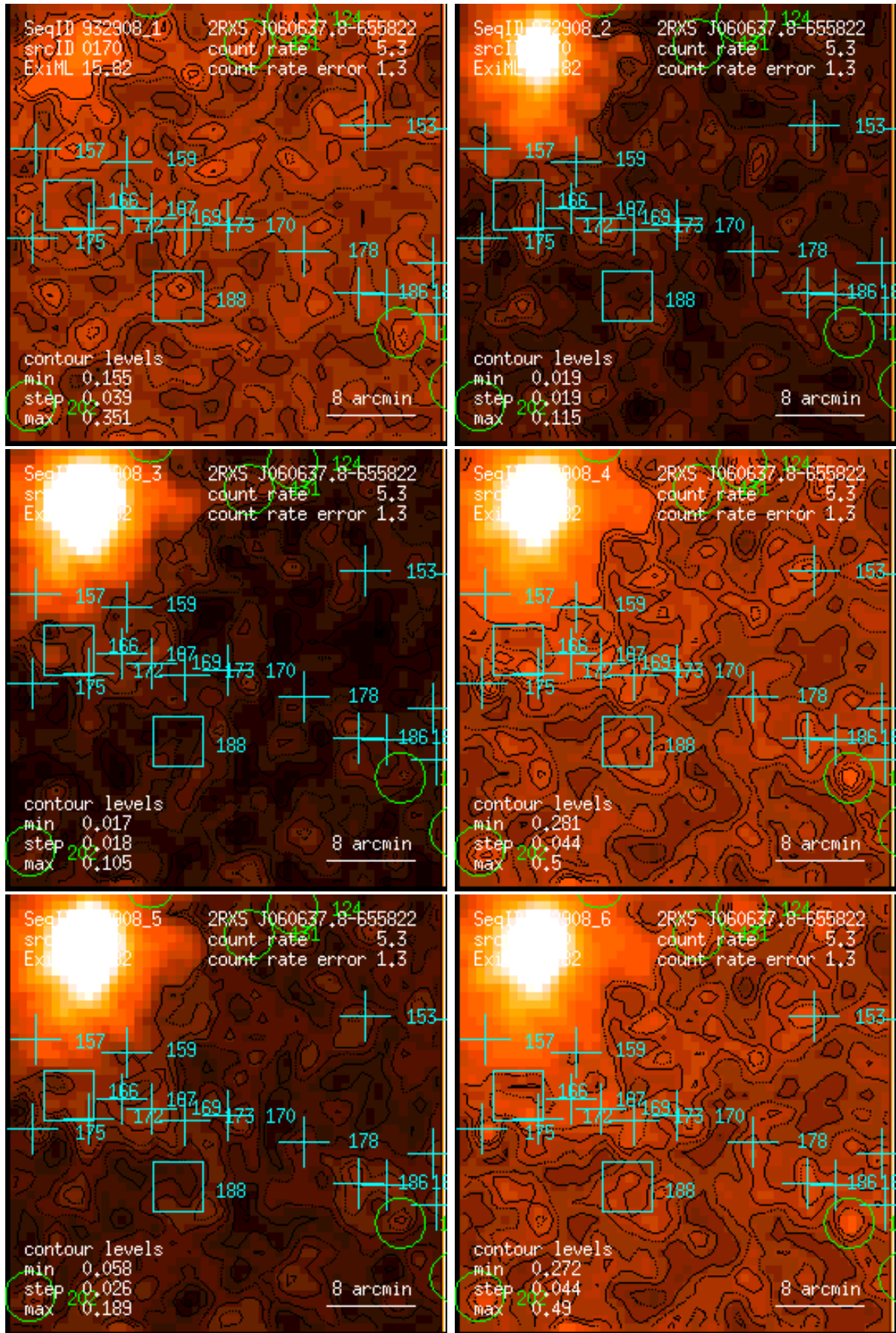
Figure 170: RASS 932908: detection 0170: band rate images, Gaussian filter: (1) PSPC channels 11 – 41, (2) 52 – 90, (3) 91 – 201, (4) 11 – 235, (5) 52 – 201, (6) 11 – 201. Broad band rates in counts/ks. Band rate contour levels in counts/ks/arcmin 2 .
