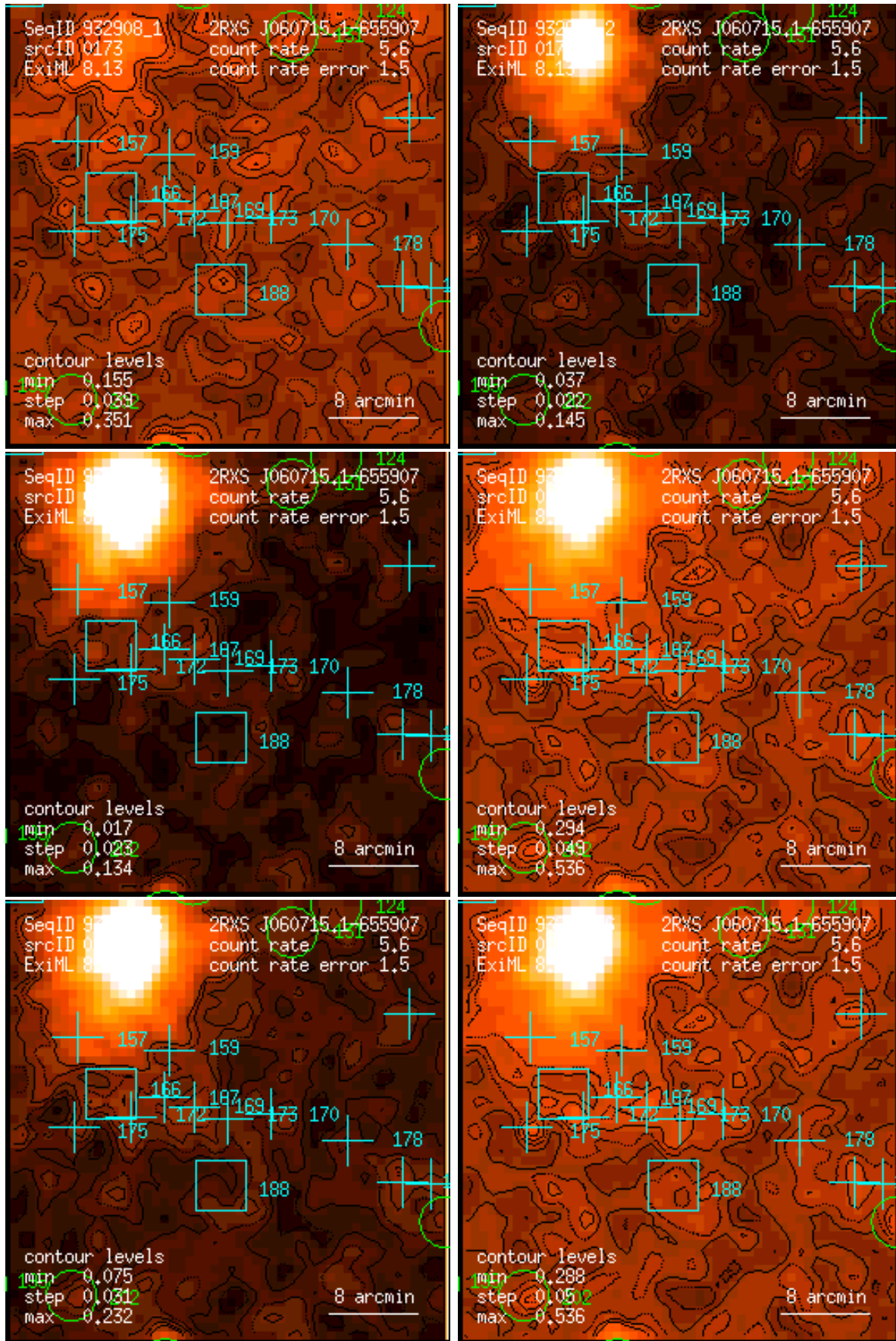
Figure 173: RASS 932908: detection 0173: band rate images, Gaussian filter: (1) PSPC channels 11 – 41, (2) 52 – 90, (3) 91 – 201, (4) 11 – 235, (5) 52 – 201, (6) 11 – 201. Broad band rates in counts/ks. Band rate contour levels in counts/ks/arcmin 2 .
