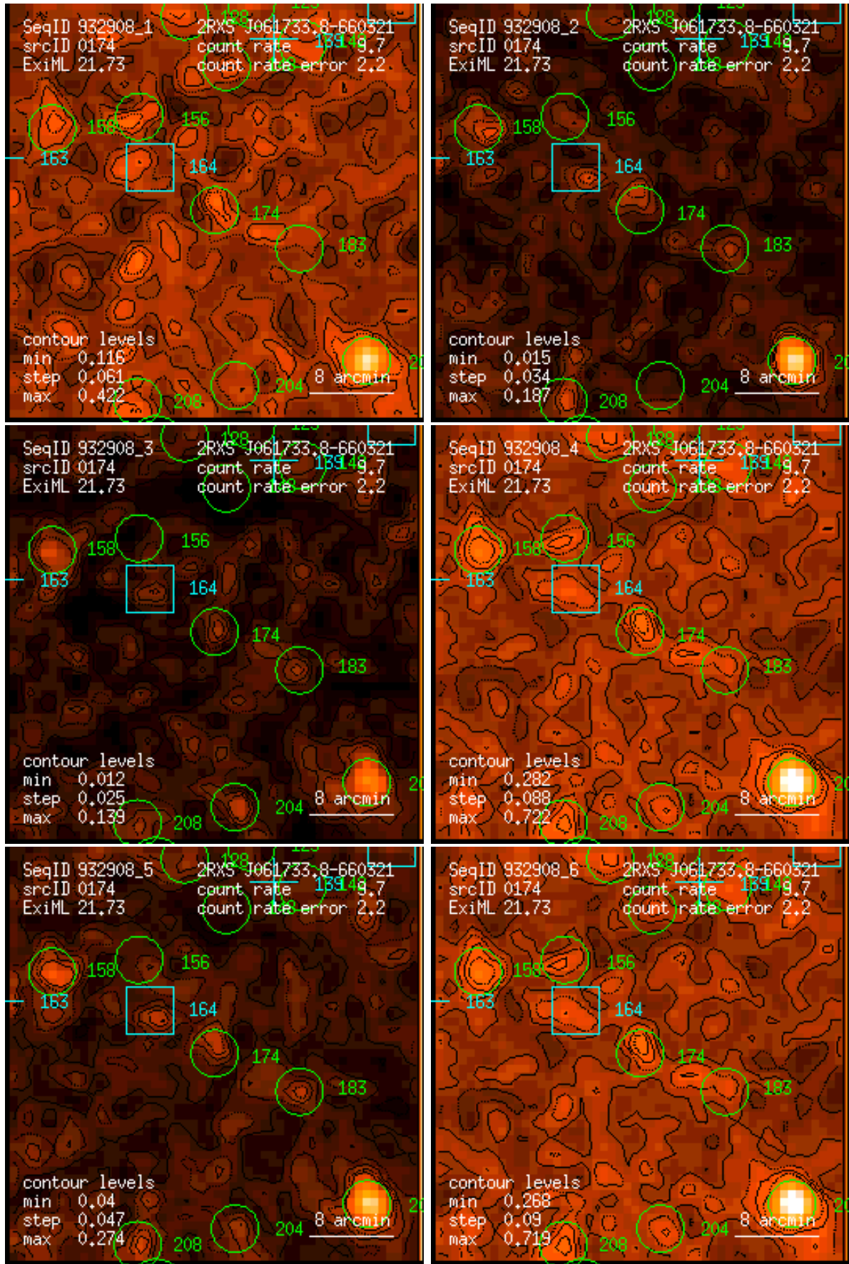
Figure 174: RASS 932908: detection 0174: band rate images, Gaussian filter: (1) PSPC channels 11 – 41, (2) 52 – 90, (3) 91 – 201, (4) 11 – 235, (5) 52 – 201, (6) 11 – 201. Broad band rates in counts/ks. Band rate contour levels in counts/ks/arcmin 2 .
