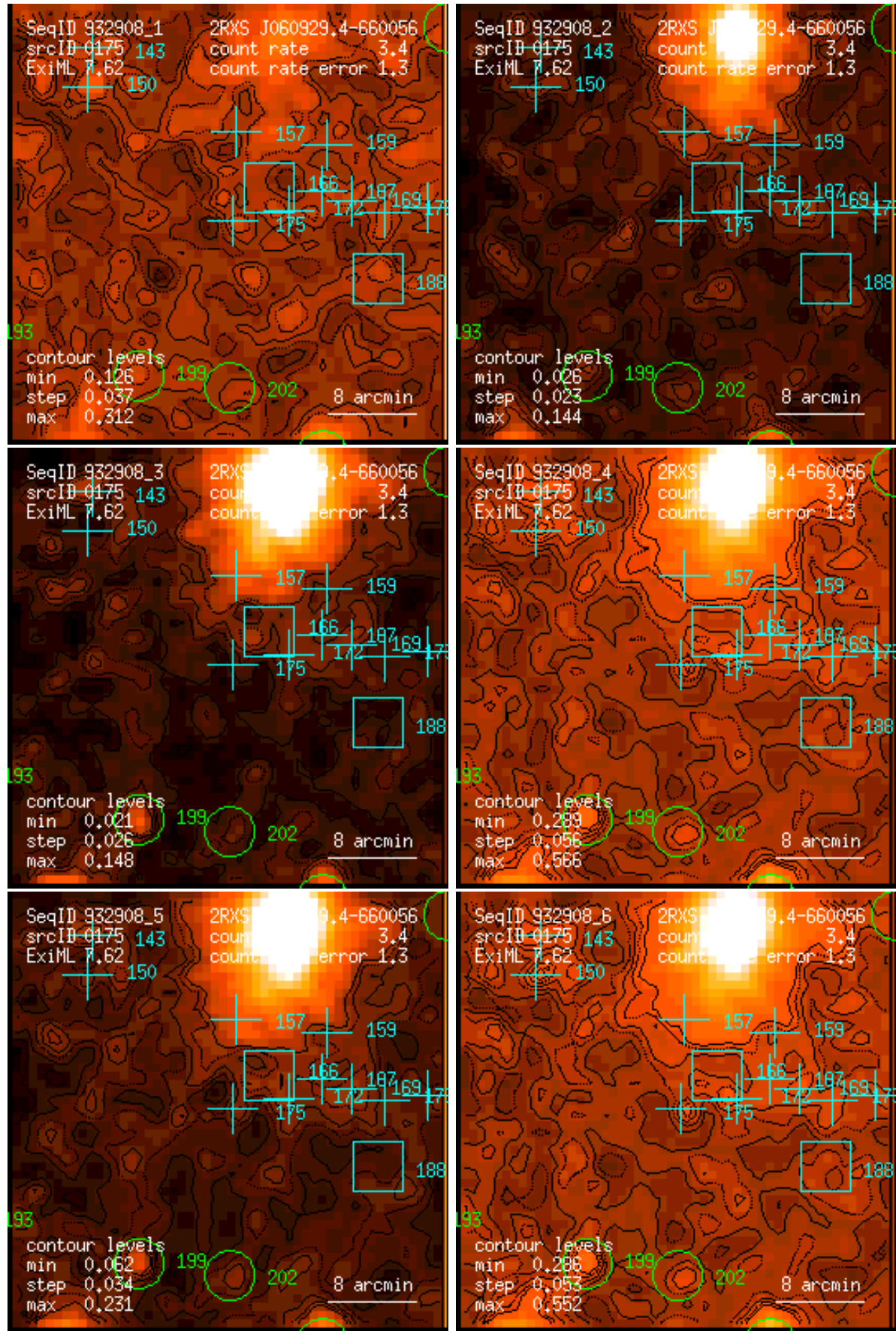
Figure 175: RASS 932908: detection 0175: band rate images, Gaussian filter: (1) PSPC channels 11 – 41, (2) 52 – 90, (3) 91 – 201, (4) 11 – 235, (5) 52 – 201, (6) 11 – 201. Broad band rates in counts/ks. Band rate contour levels in counts/ks/arcmin 2 .
