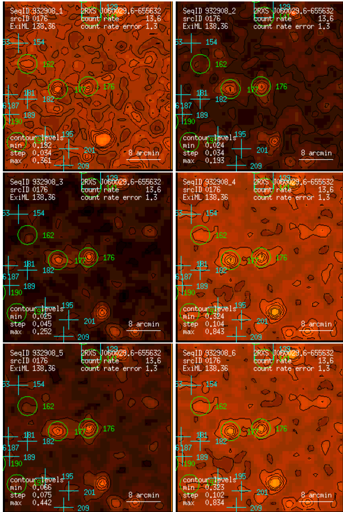
Figure 176: RASS 932908: detection 0176: band rate images, Gaussian filter: (1) PSPC channels 11 – 41, (2) 52 – 90, (3) 91 – 201, (4) 11 – 235, (5) 52 – 201, (6) 11 – 201. Broad band rates in counts/ks. Band rate contour levels in counts/ks/arcmin 2 .
