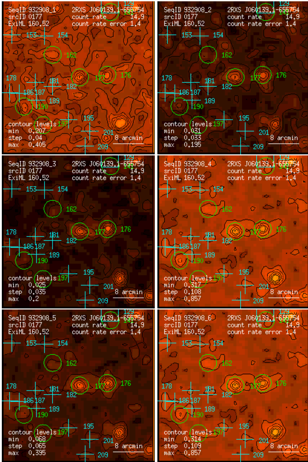
Figure 177: RASS 932908: detection 0177: band rate images, Gaussian filter: (1) PSPC channels 11 – 41, (2) 52 – 90, (3) 91 – 201, (4) 11 – 235, (5) 52 – 201, (6) 11 – 201. Broad band rates in counts/ks. Band rate contour levels in counts/ks/arcmin 2 .
