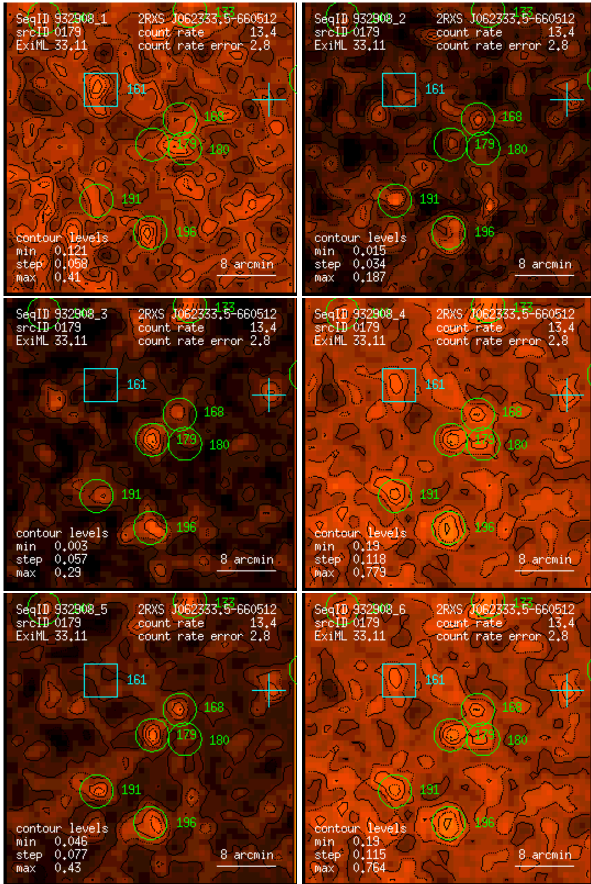
Figure 179: RASS 932908: detection 0179: band rate images, Gaussian filter: (1) PSPC channels 11 – 41, (2) 52 – 90, (3) 91 – 201, (4) 11 – 235, (5) 52 – 201, (6) 11 – 201. Broad band rates in counts/ks. Band rate contour levels in counts/ks/arcmin 2 .
