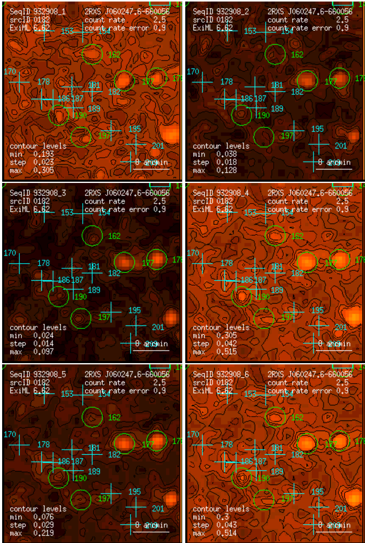
Figure 182: RASS 932908: detection 0182: band rate images, Gaussian filter: (1) PSPC channels 11 – 41, (2) 52 – 90, (3) 91 – 201, (4) 11 – 235, (5) 52 – 201, (6) 11 – 201. Broad band rates in counts/ks. Band rate contour levels in counts/ks/arcmin 2 .
