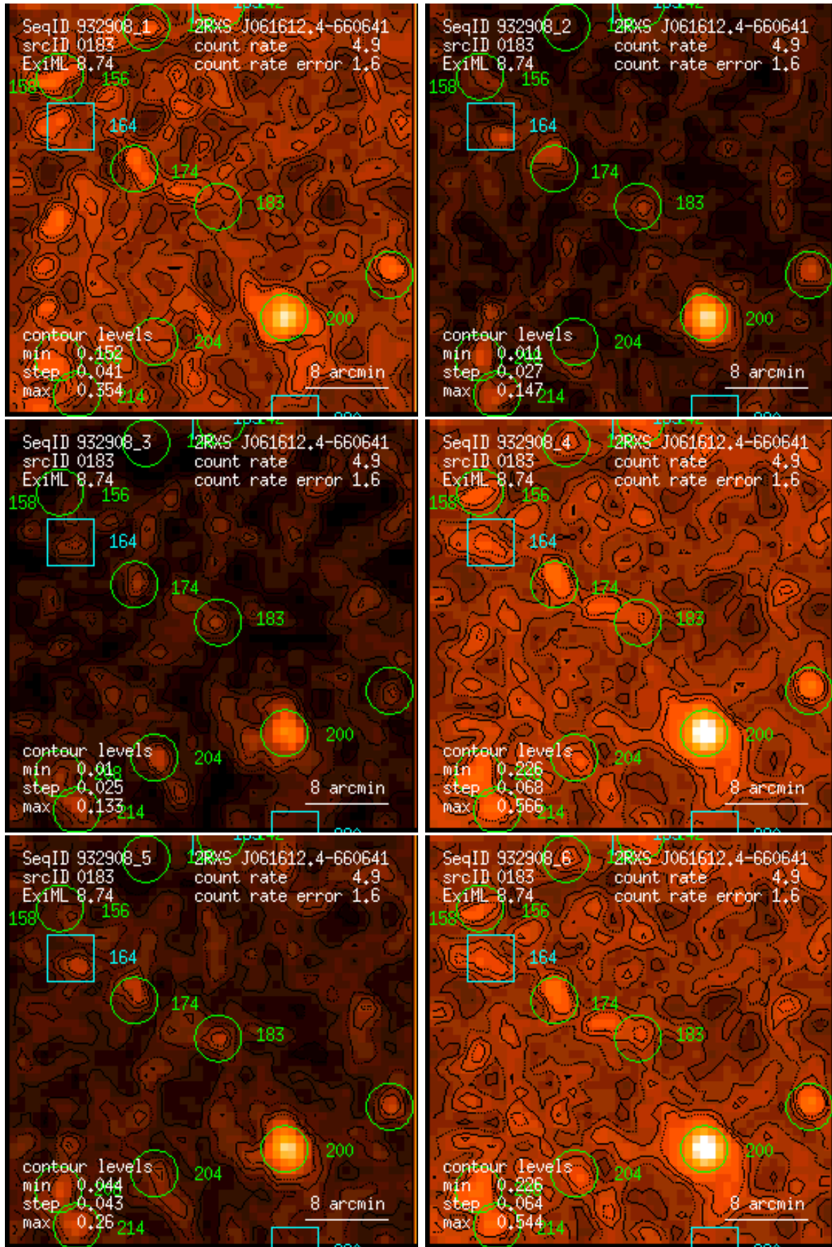
Figure 183: RASS 932908: detection 0183: band rate images, Gaussian filter: (1) PSPC channels 11 – 41, (2) 52 – 90, (3) 91 – 201, (4) 11 – 235, (5) 52 – 201, (6) 11 – 201. Broad band rates in counts/ks. Band rate contour levels in counts/ks/arcmin 2 .
