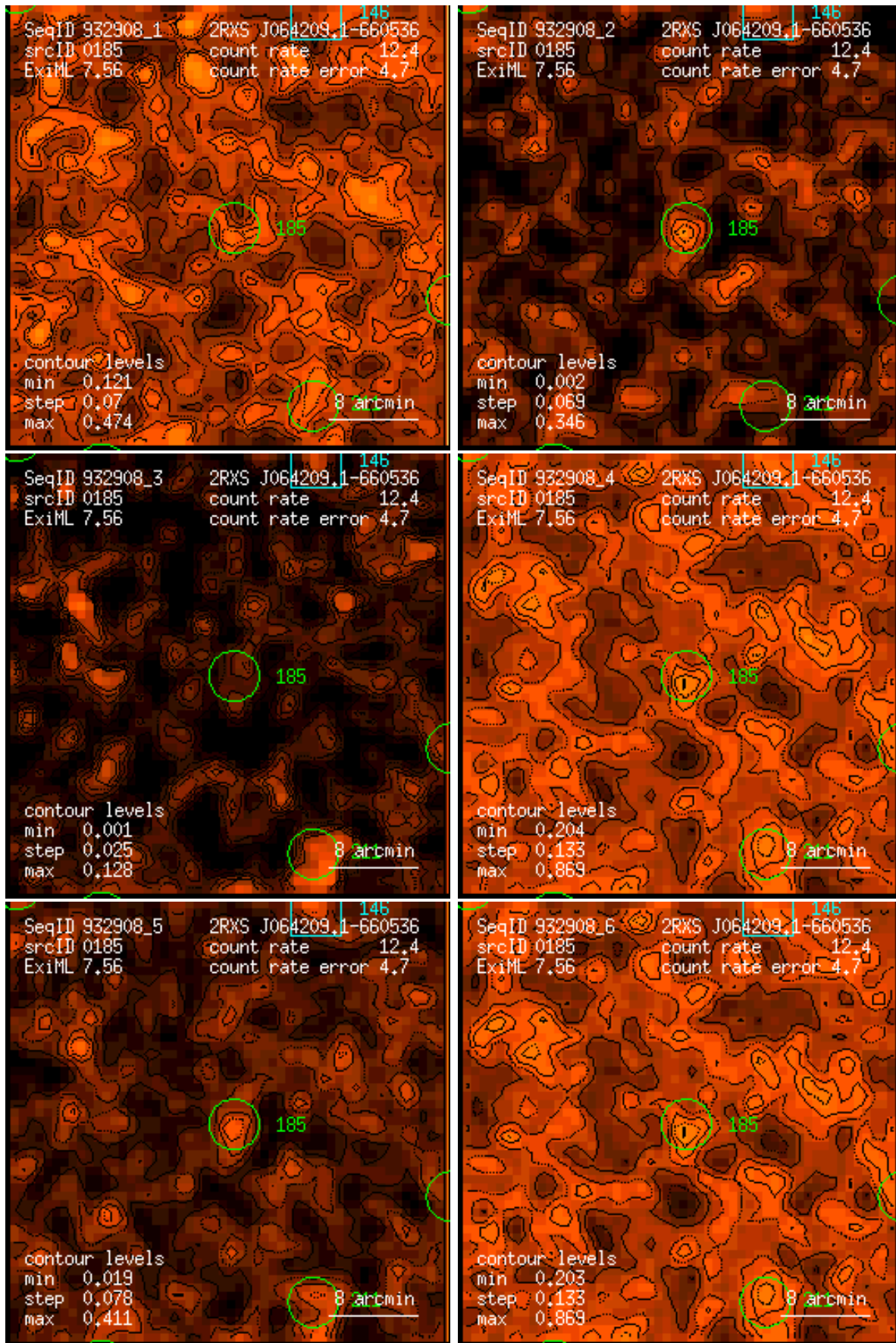
Figure 185: RASS 932908: detection 0185: band rate images, Gaussian filter: (1) PSPC channels 11 – 41, (2) 52 – 90, (3) 91 – 201, (4) 11 – 235, (5) 52 – 201, (6) 11 – 201. Broad band rates in counts/ks. Band rate contour levels in counts/ks/arcmin 2 .
