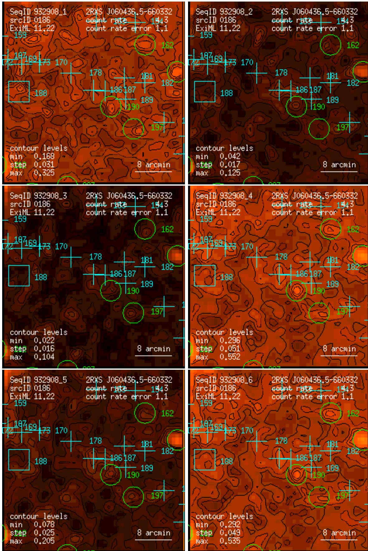
Figure 186: RASS 932908: detection 0186: band rate images, Gaussian filter: (1) PSPC channels 11 – 41, (2) 52 – 90, (3) 91 – 201, (4) 11 – 235, (5) 52 – 201, (6) 11 – 201. Broad band rates in counts/ks. Band rate contour levels in counts/ks/arcmin 2 .
