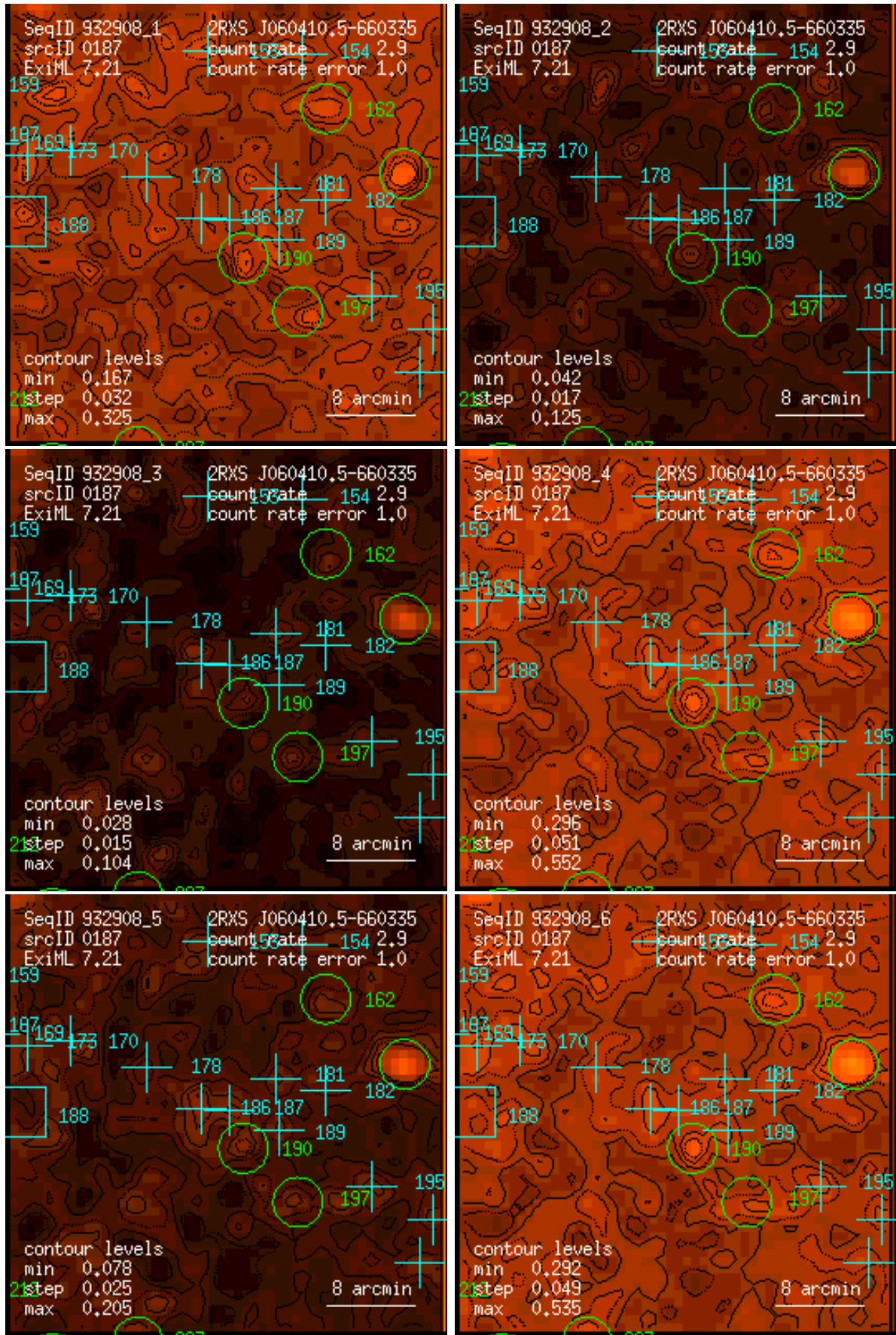
Figure 187: RASS 932908: detection 0187: band rate images, Gaussian filter: (1) PSPC channels 11 – 41, (2) 52 – 90, (3) 91 – 201, (4) 11 – 235, (5) 52 – 201, (6) 11 – 201. Broad band rates in counts/ks. Band rate contour levels in counts/ks/arcmin 2 .
