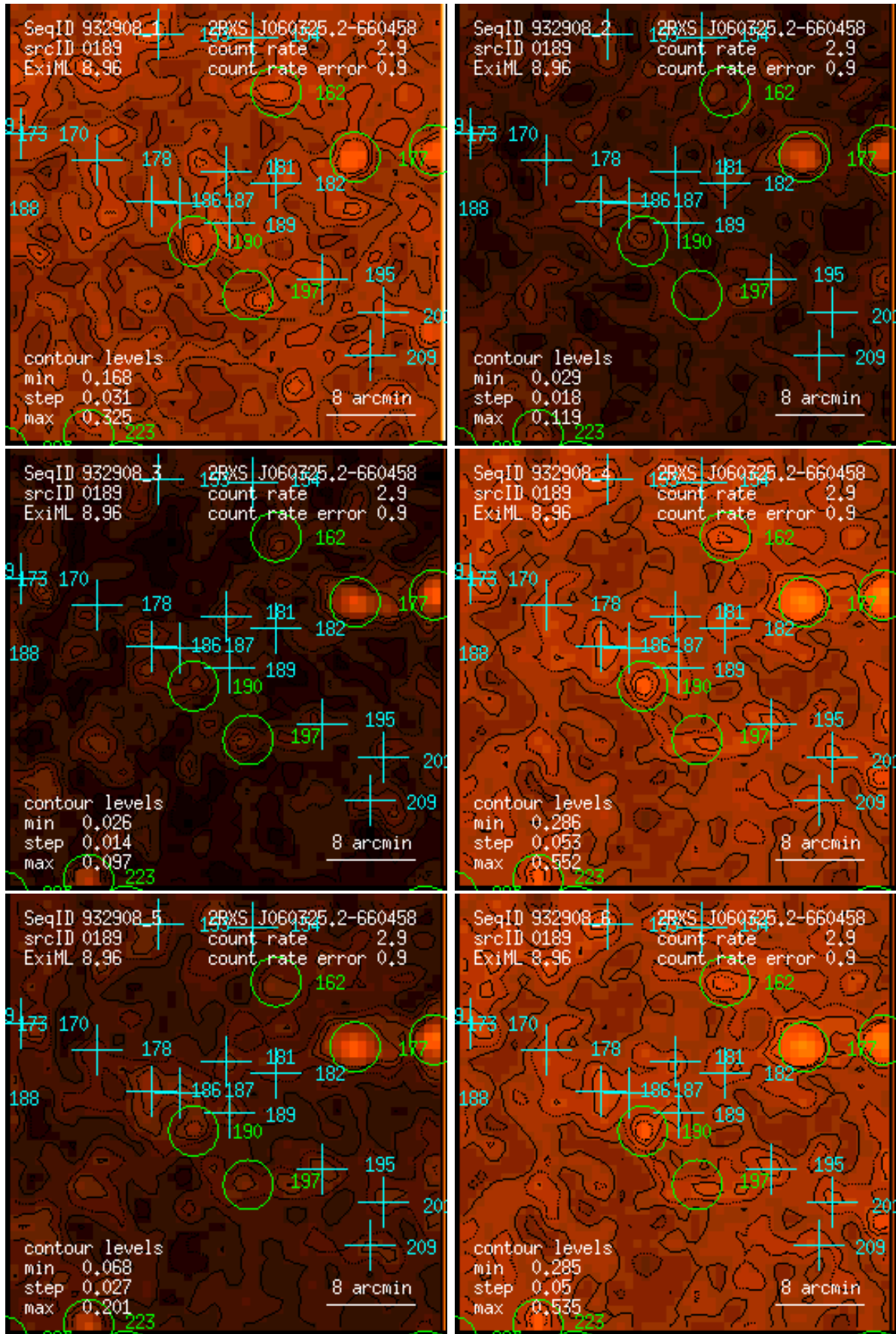
Figure 189: RASS 932908: detection 0189: band rate images, Gaussian filter: (1) PSPC channels 11 – 41, (2) 52 – 90, (3) 91 – 201, (4) 11 – 235, (5) 52 – 201, (6) 11 – 201. Broad band rates in counts/ks. Band rate contour levels in counts/ks/arcmin 2 .
